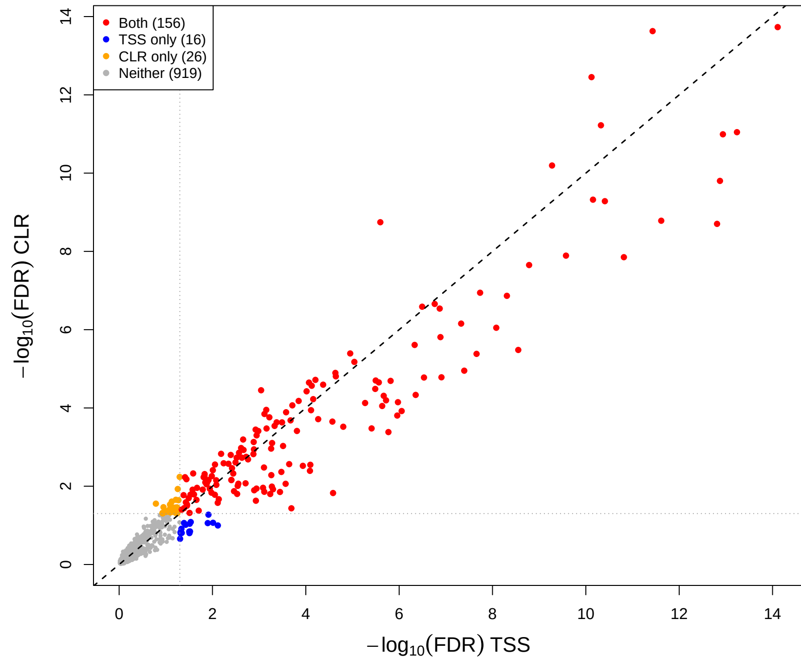
cent vs mage – CLR(const=0) vs TSS (gamma = 0.3)
