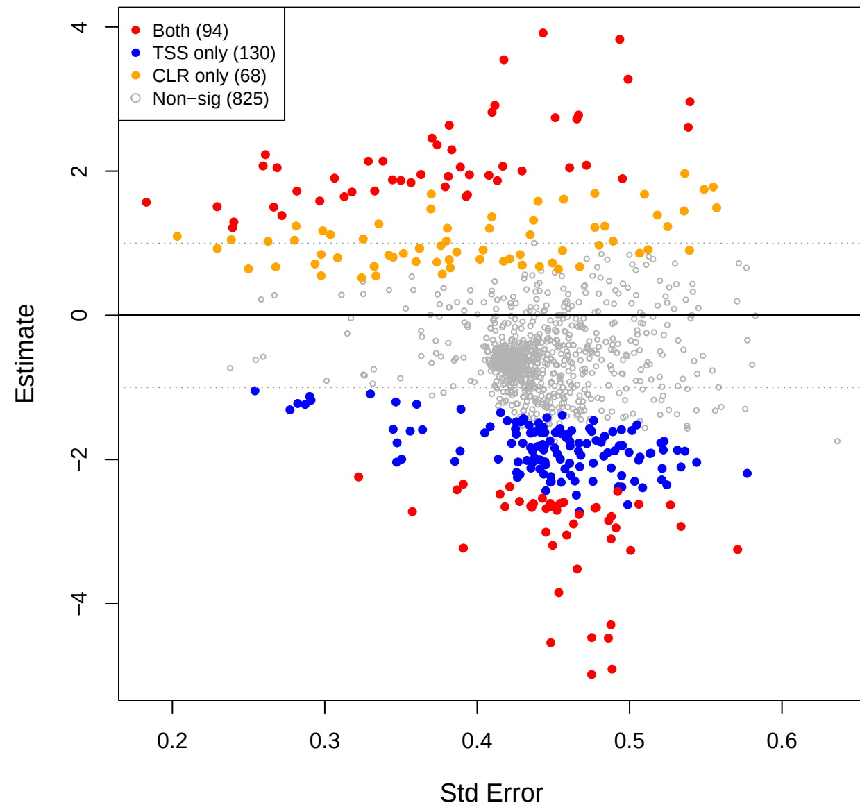
cent vs mage – TSS(const=-0.3) effect space
