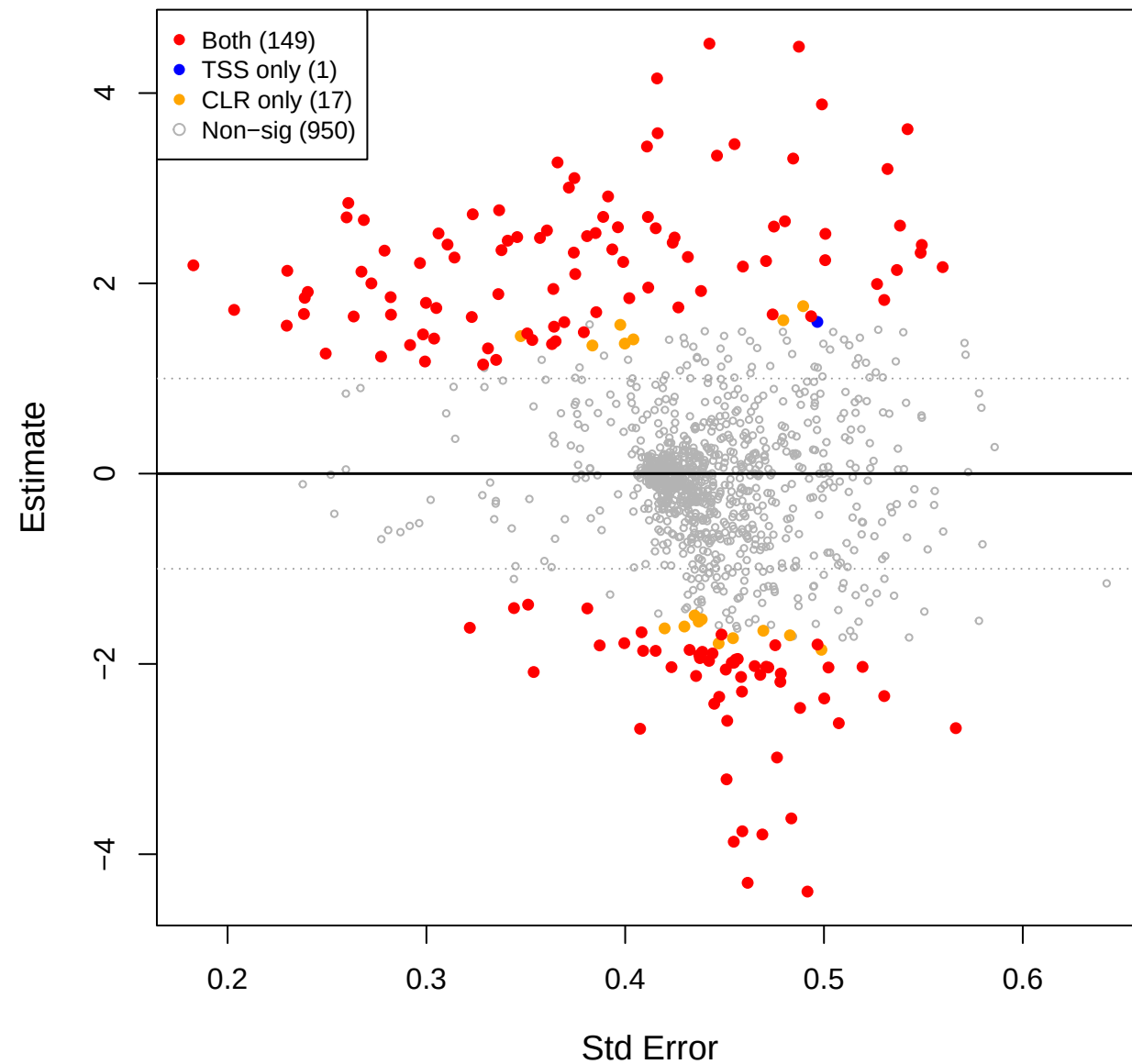
cent vs mage – TSS(const=0.4) effect space
