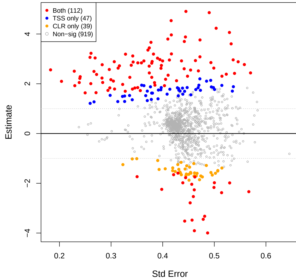
cent vs mage – TSS(const=0.7) effect space
