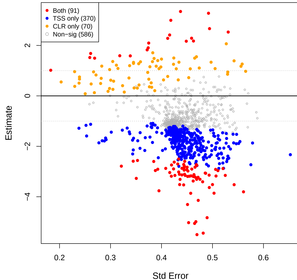
cent vs mage – TSS(const=-0.8) effect space
