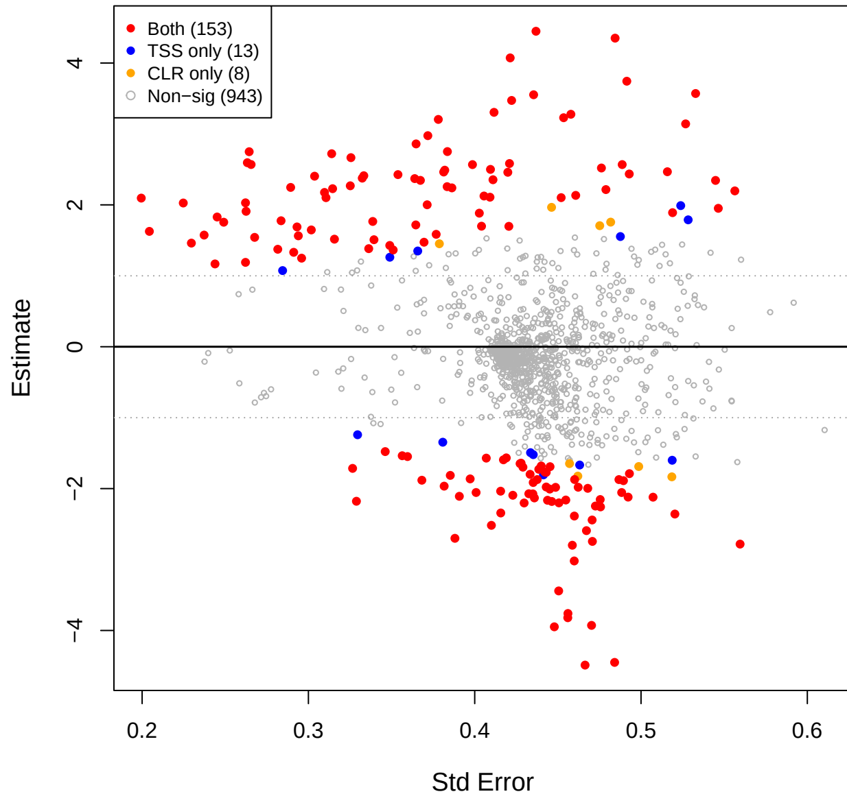
cent vs mage – CLR effect space
