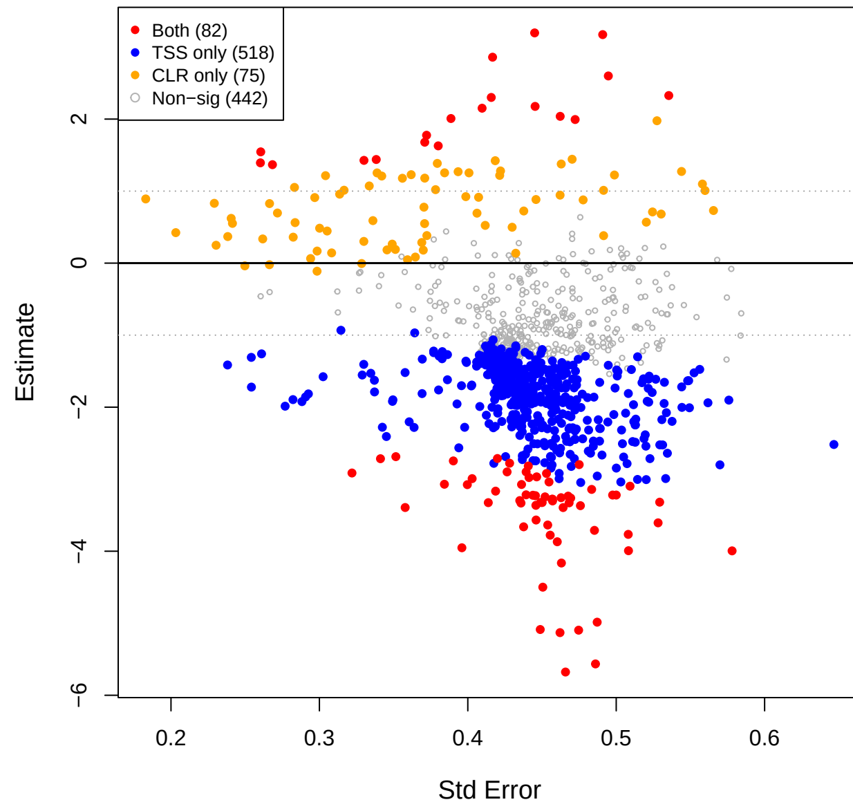
cent vs mage – TSS(const=-1) effect space
