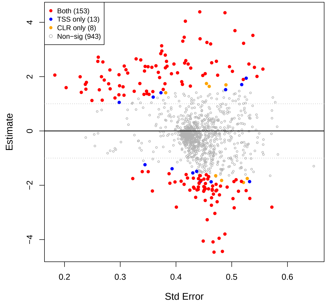
cent vs mage – TSS(const=0.2) effect space
