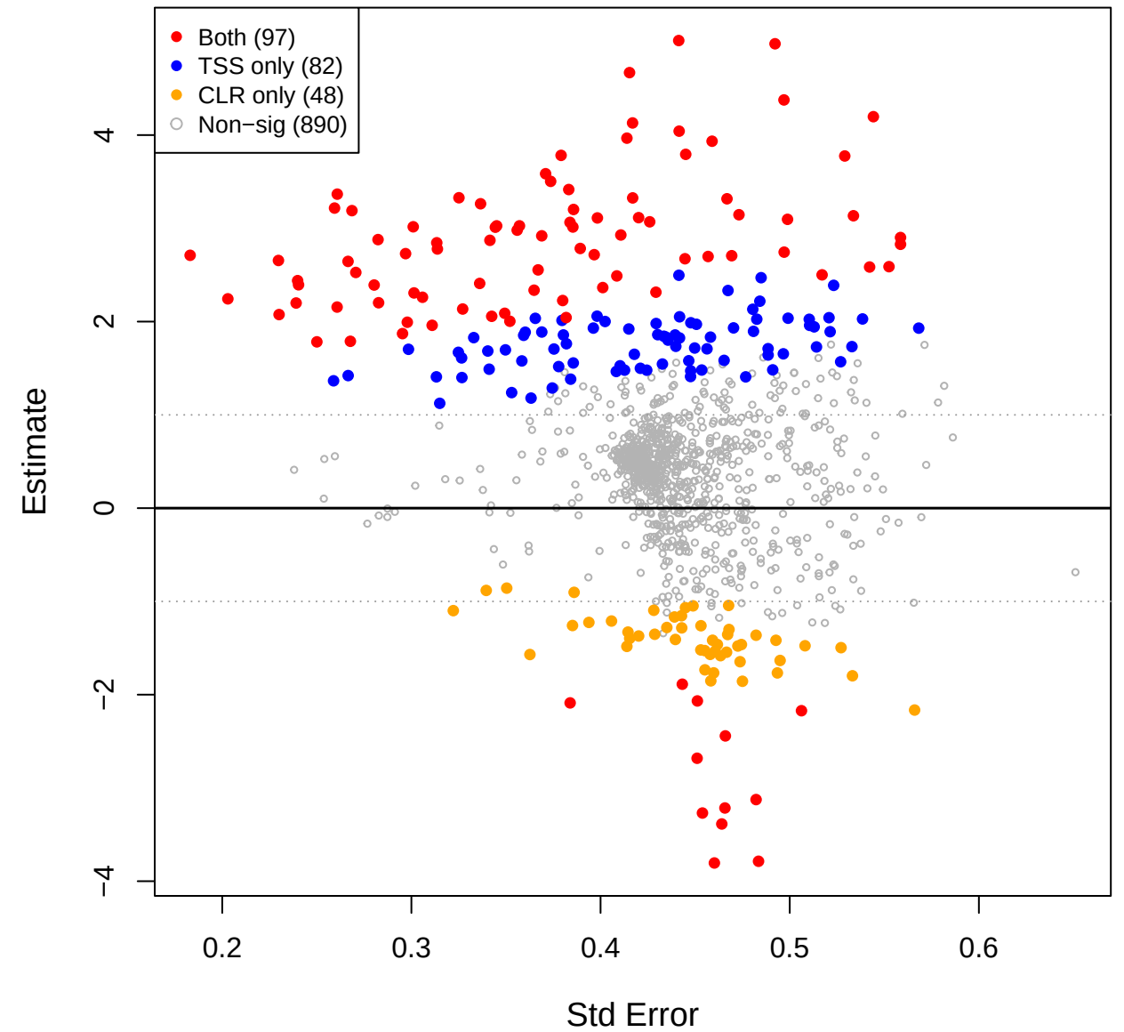
cent vs mage – TSS(const=0.9) effect space
