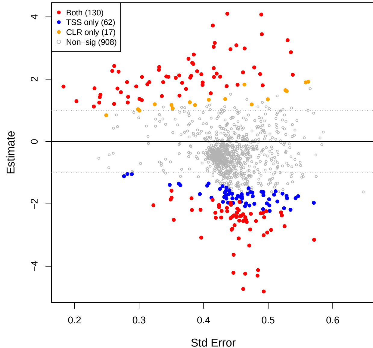
cent vs mage – TSS(const=-0.1) effect space
