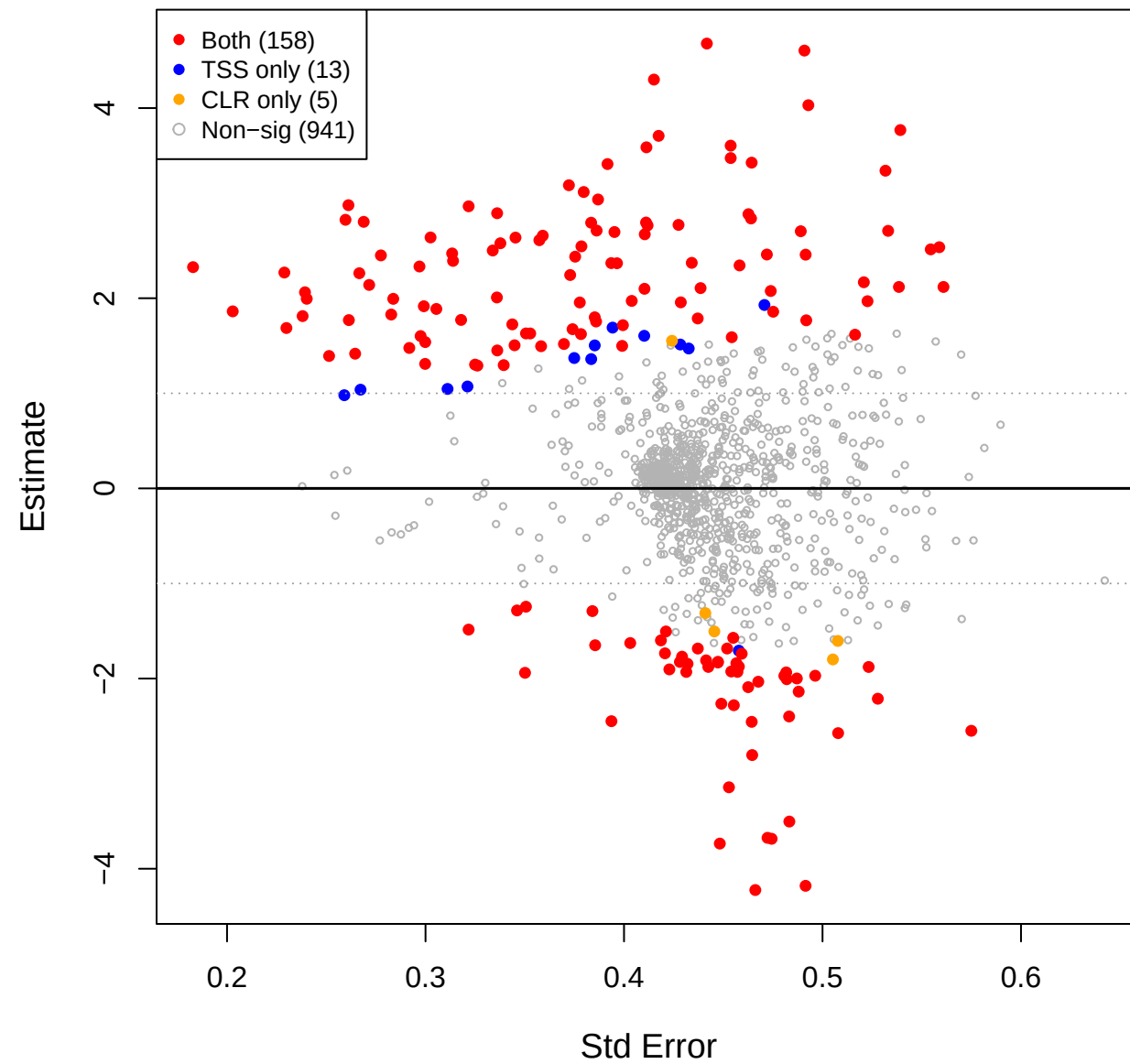
cent vs mage – TSS(const=0.5) effect space
