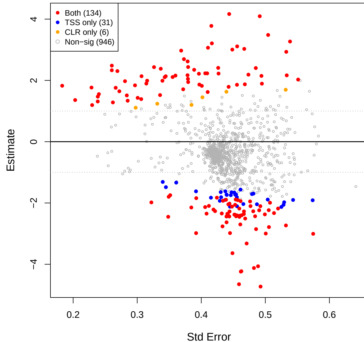
cent vs mage – TSS(const=0) effect space
