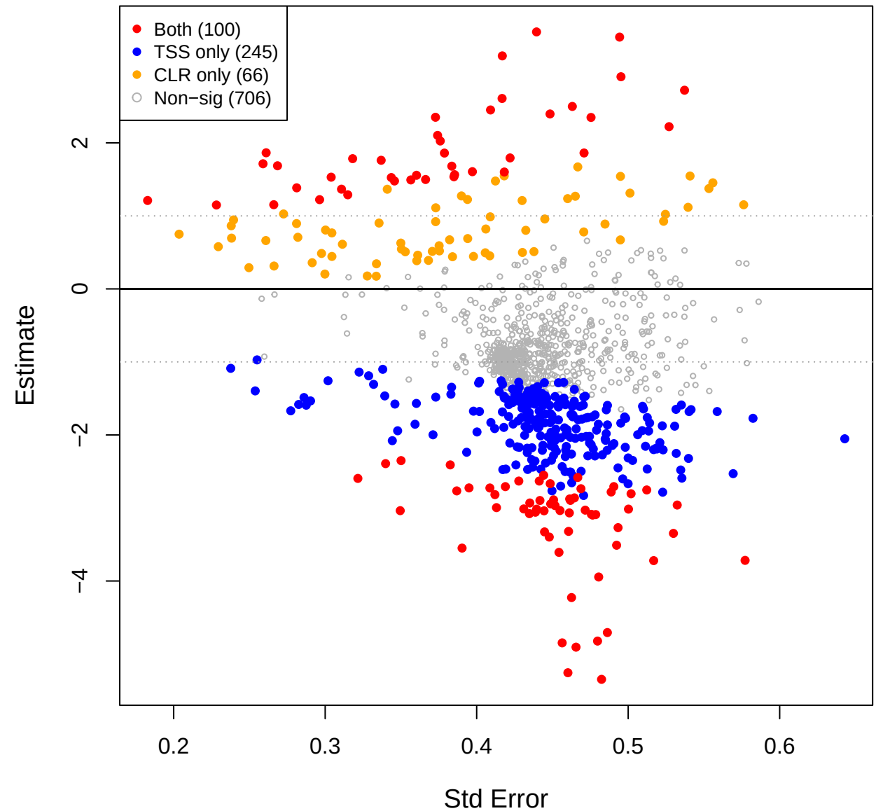
cent vs mage – TSS(const=-0.6) effect space
