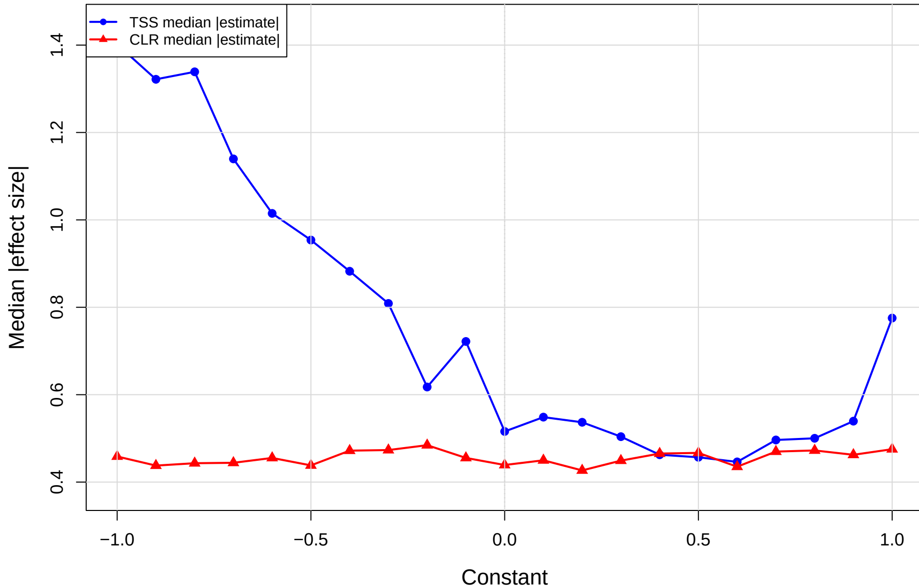
TSS_const | cent vs mage | gamma=0.5 Median absolute effect size across all features
