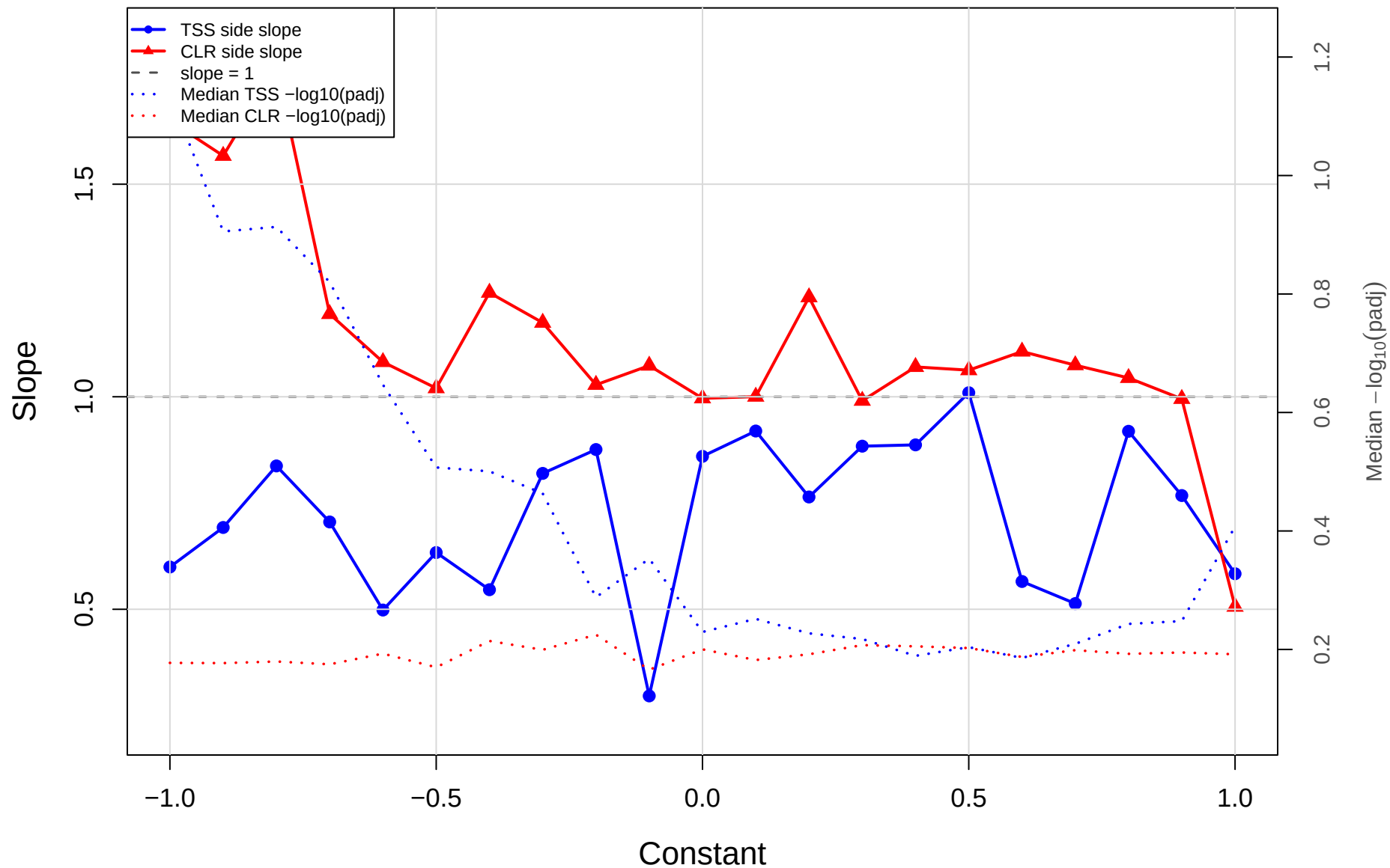
TSS_const | cent vs mage | gamma=0.5 Slope of red-dot regression
