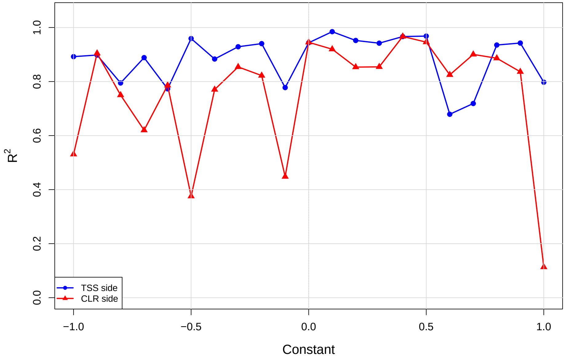
TSS_const | cent vs mage | gamma=0.5 R-squared of red-dot regression
