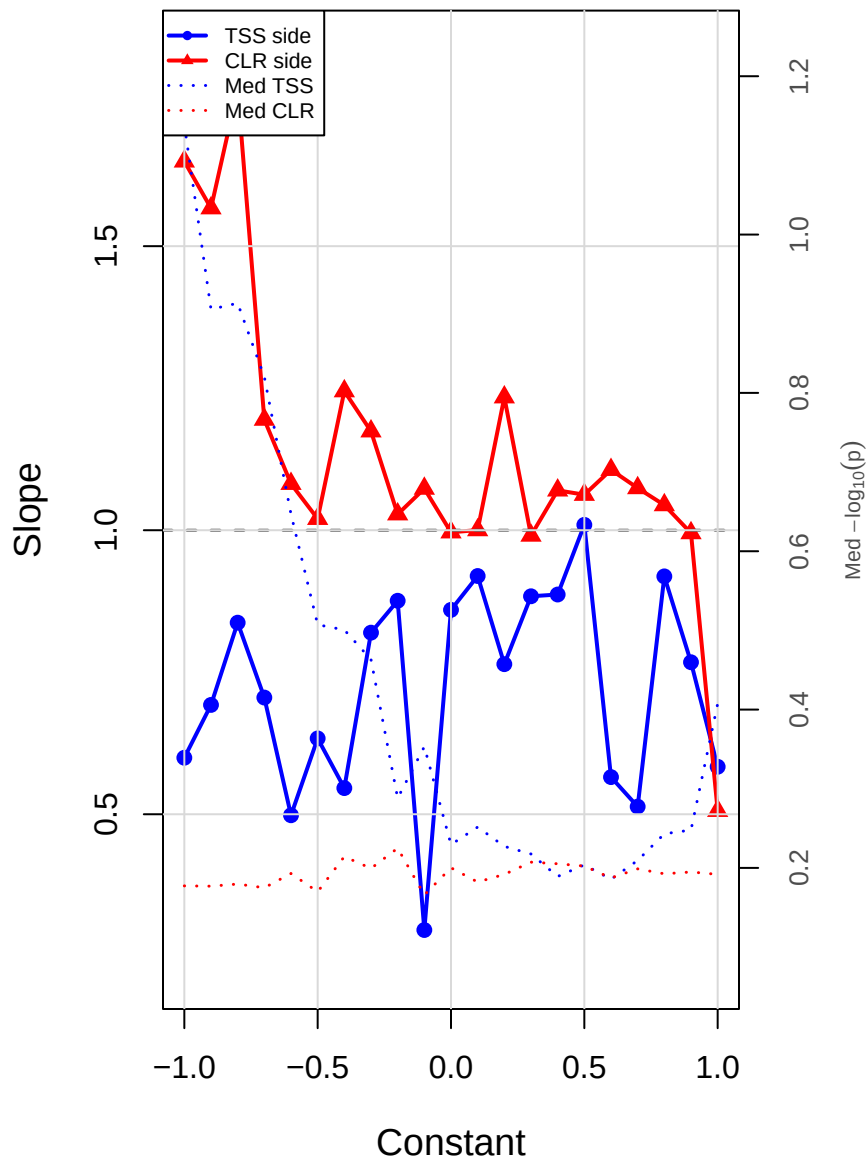
TSS_const | cent vs mage | gamma=0.5
