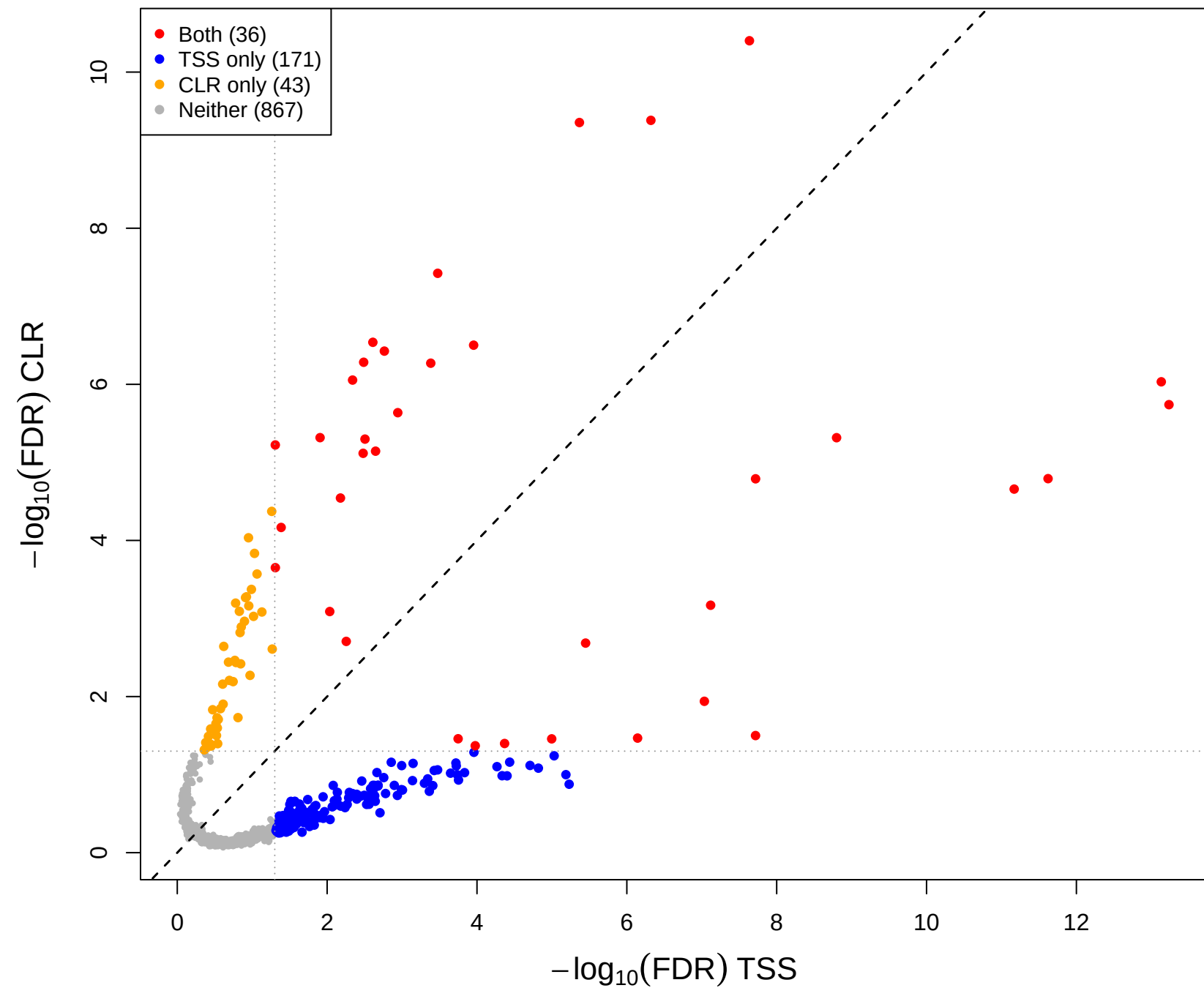
cent vs mage – CLR vs TSS(const=-0.6) (gamma = 0.5)
