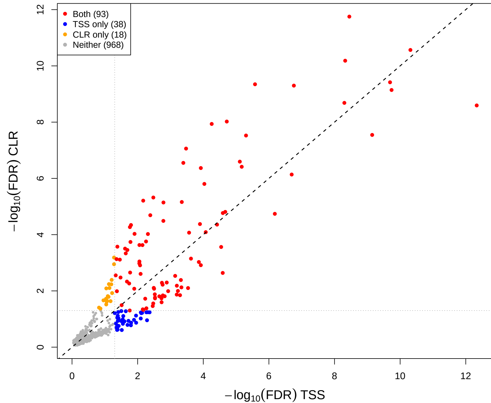
cent vs mage – CLR vs TSS(const=-0.2) (gamma = 0.5)
