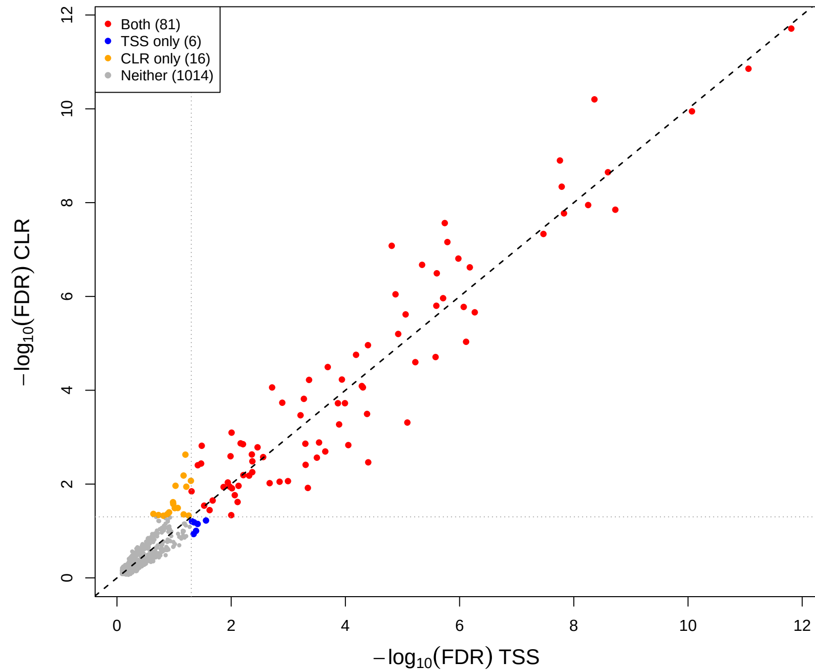
cent vs mage – CLR vs TSS(const=0.5) (gamma = 0.5)
