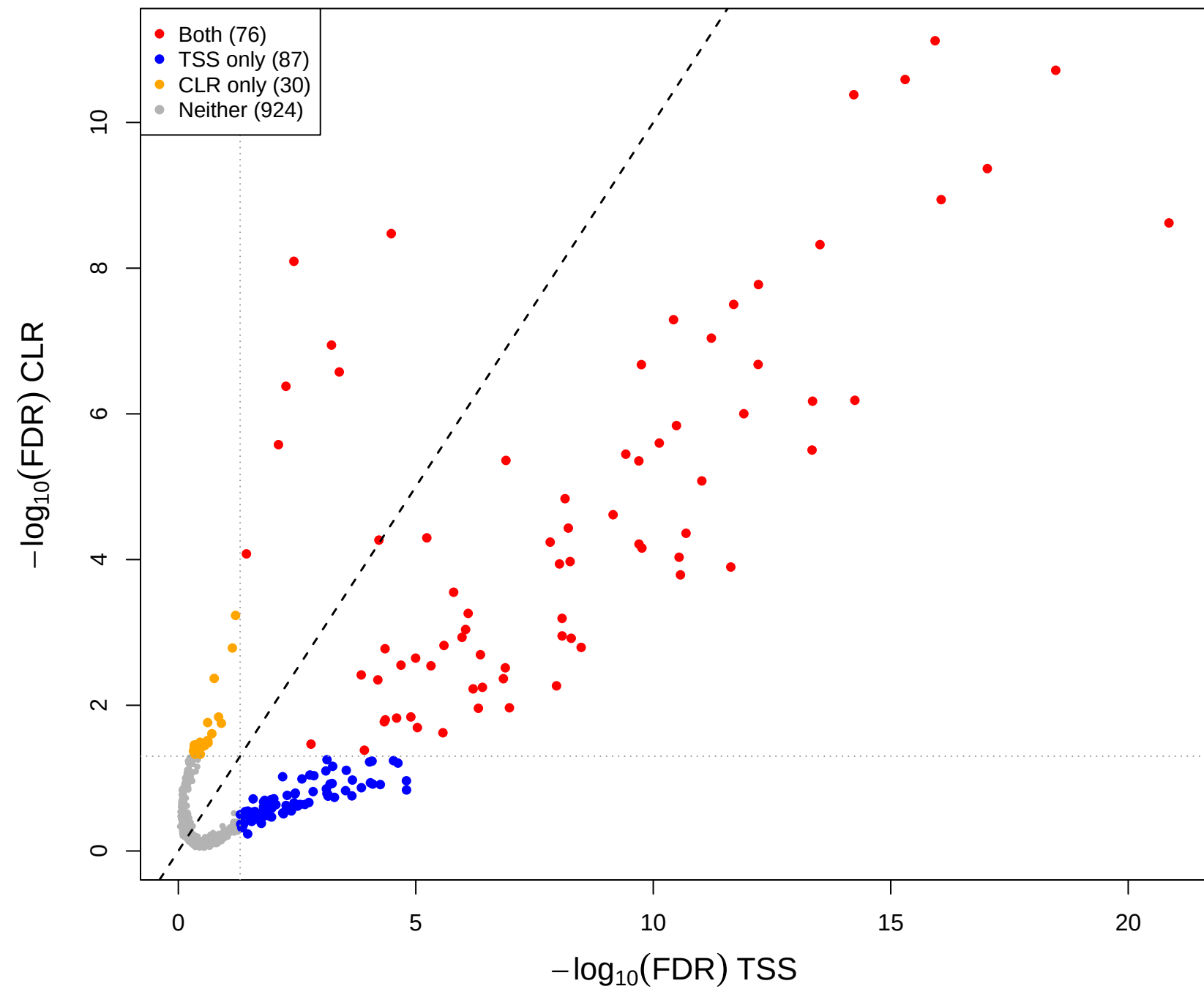
cent vs mage – CLR vs TSS(const=1) (gamma = 0.5)
