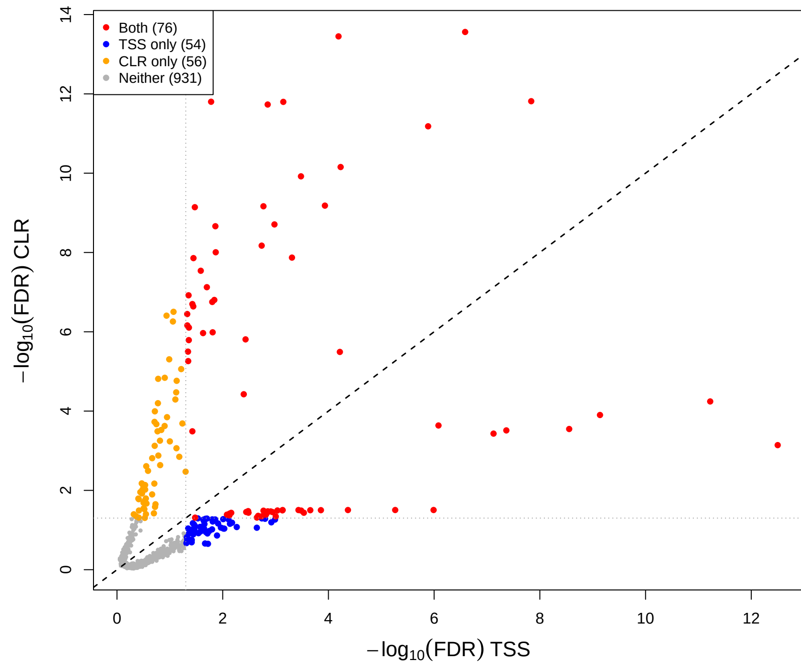
cent vs mage – CLR vs TSS(const=-0.1) (gamma = 0.5)
