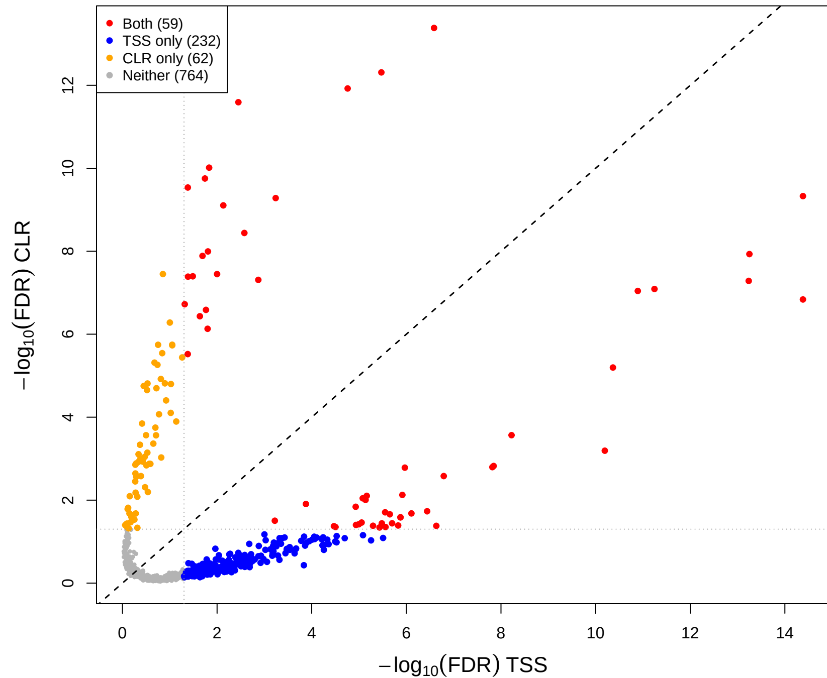
cent vs mage – CLR vs TSS(const=-0.7) (gamma = 0.5)
