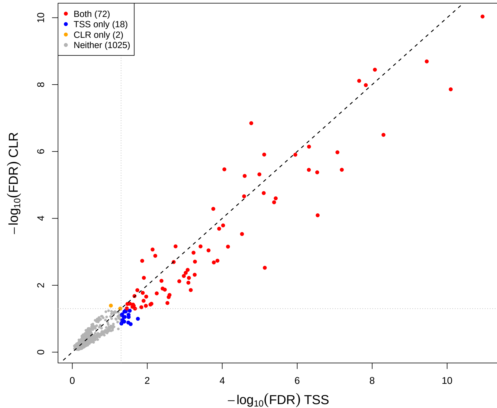
cent vs mage – CLR vs TSS(const=0) (gamma = 0.5)
