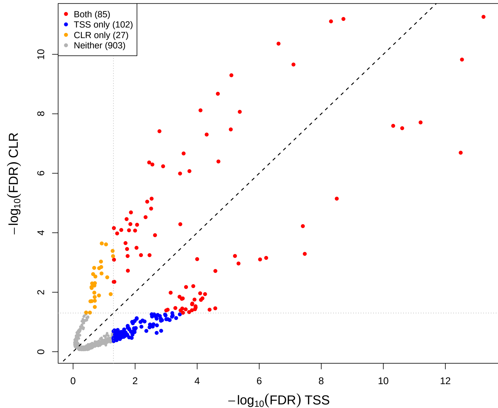
cent vs mage – CLR vs TSS(const=-0.3) (gamma = 0.5)
