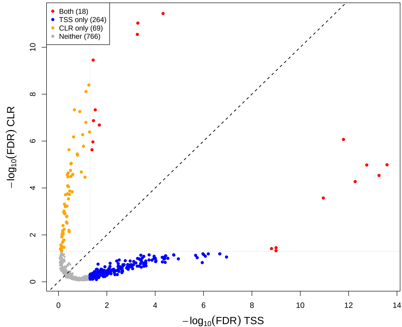
cent vs mage – CLR vs TSS(const=-0.8) (gamma = 0.5)
