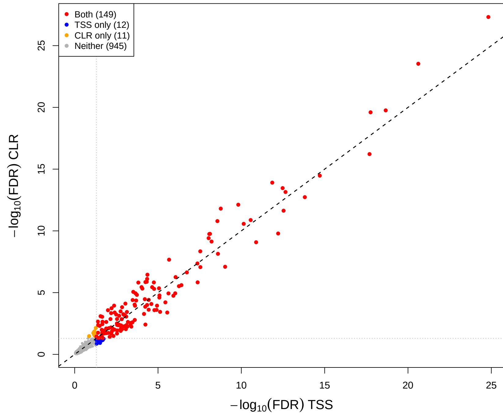
eld vs kin – CLR vs TSS(const=-0.2) (gamma = 0.5)
