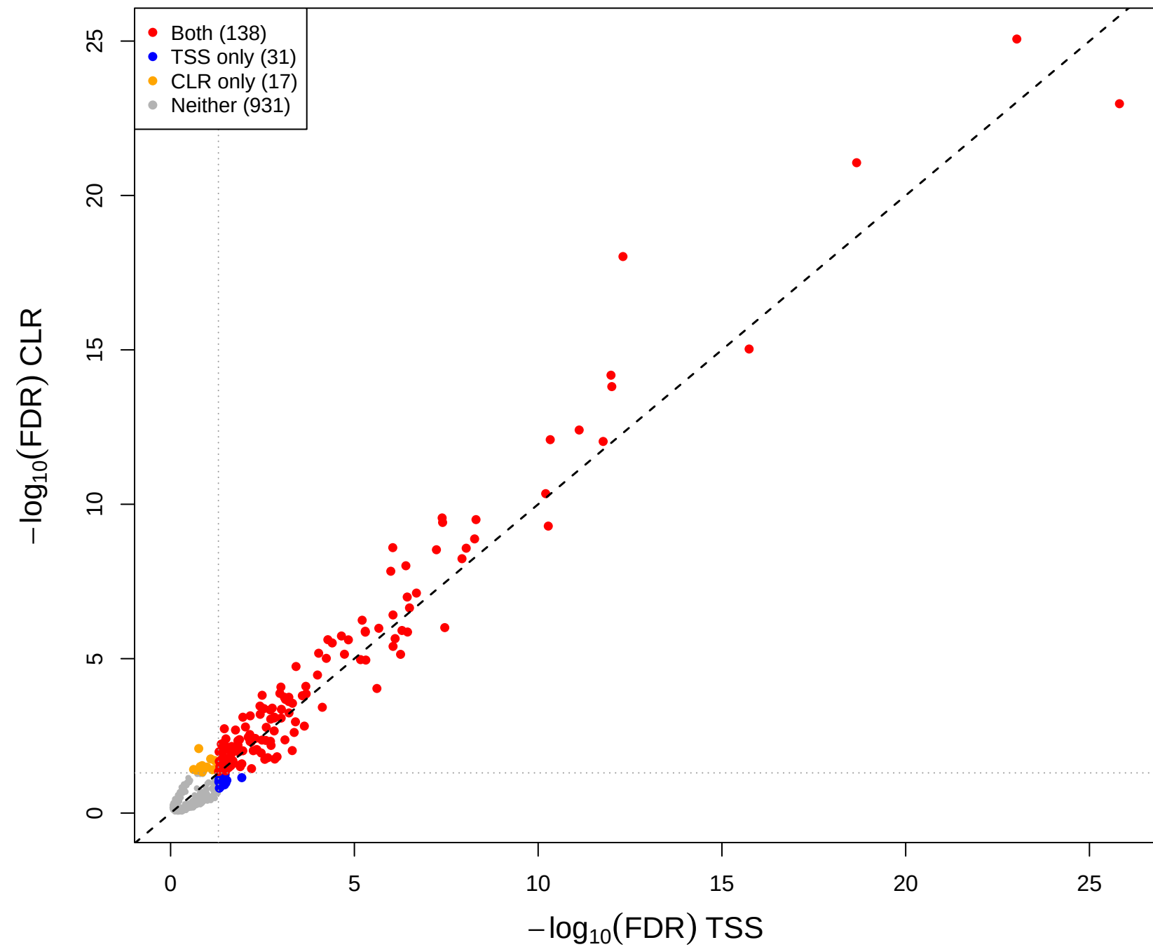
eld vs kin – CLR vs TSS(const=-0.3) (gamma = 0.5)
