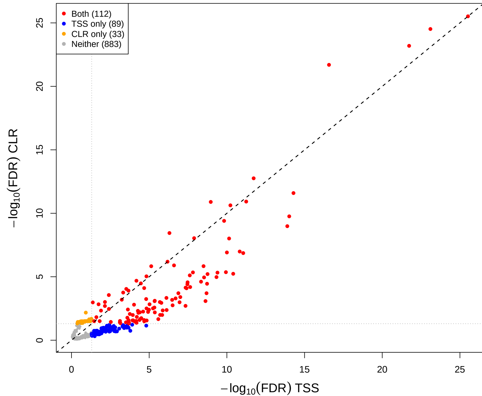
eld vs kin - CLR vs TSS(const=-0.8) (gamma = 0.5)
