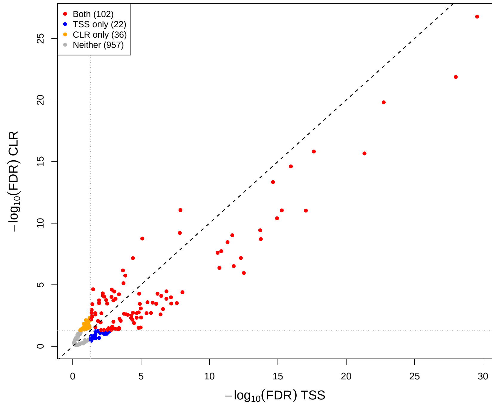
eld vs kin – CLR vs TSS(const=0.5) (gamma = 0.5)
