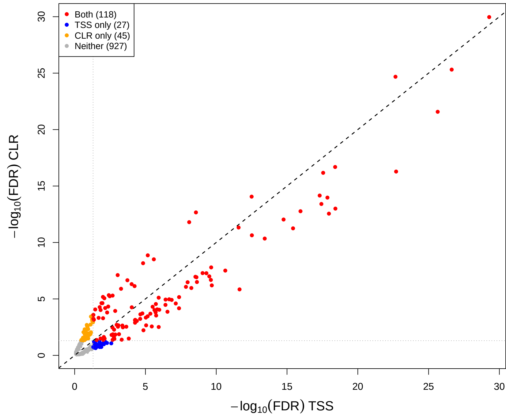
eld vs kin – CLR vs TSS(const=0.7) (gamma = 0.5)
