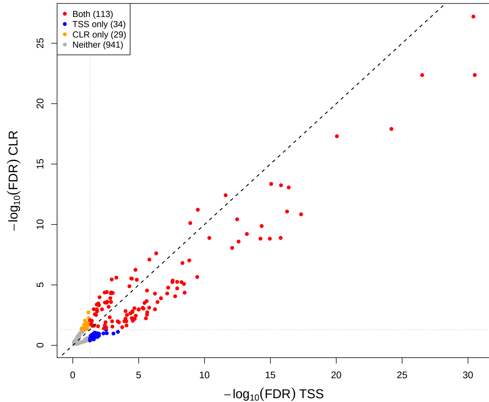
eld vs kin – CLR vs TSS(const=0.4) (gamma = 0.5)
