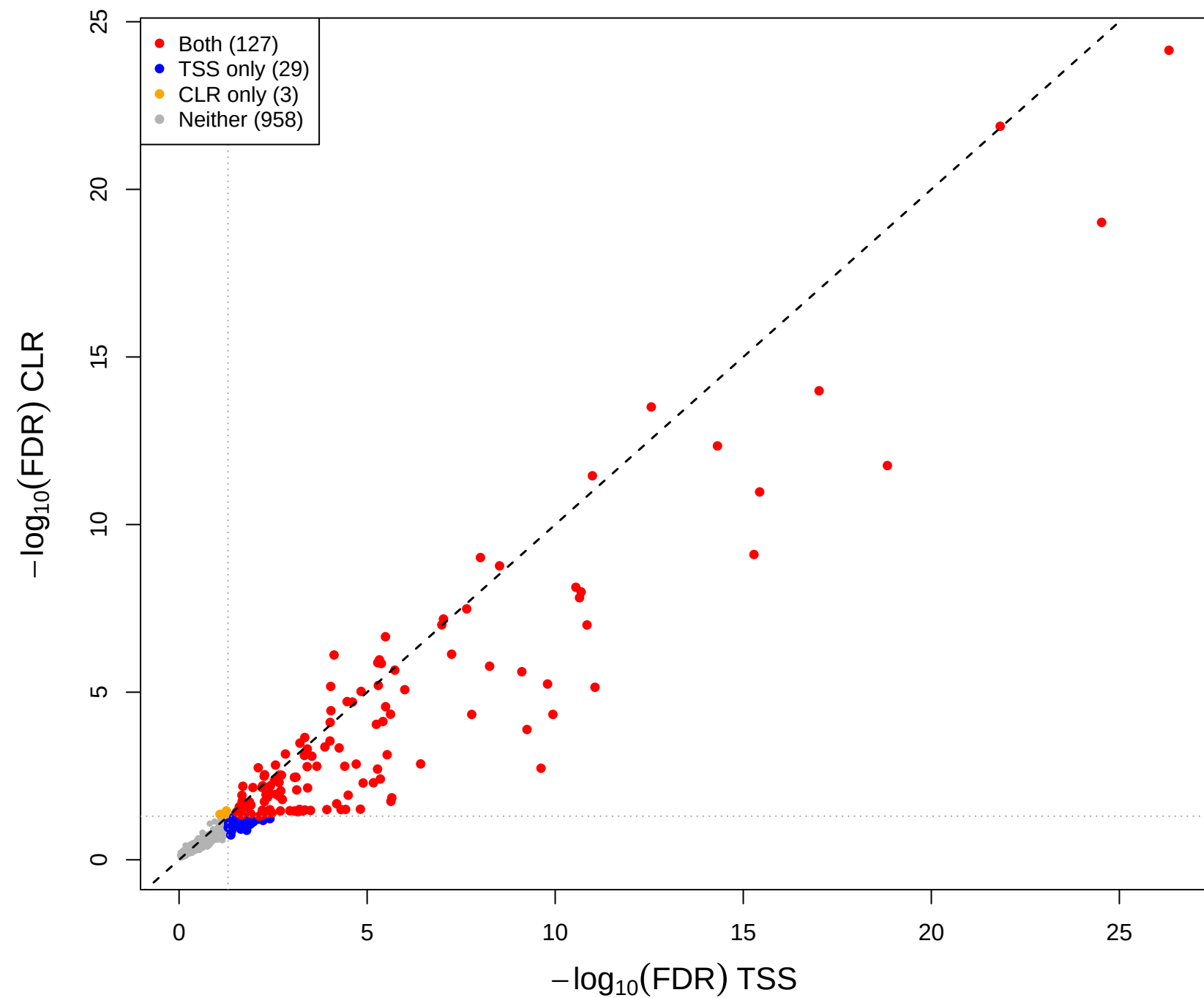
eld vs kin – CLR vs TSS(const=-0.1) (gamma = 0.5)
