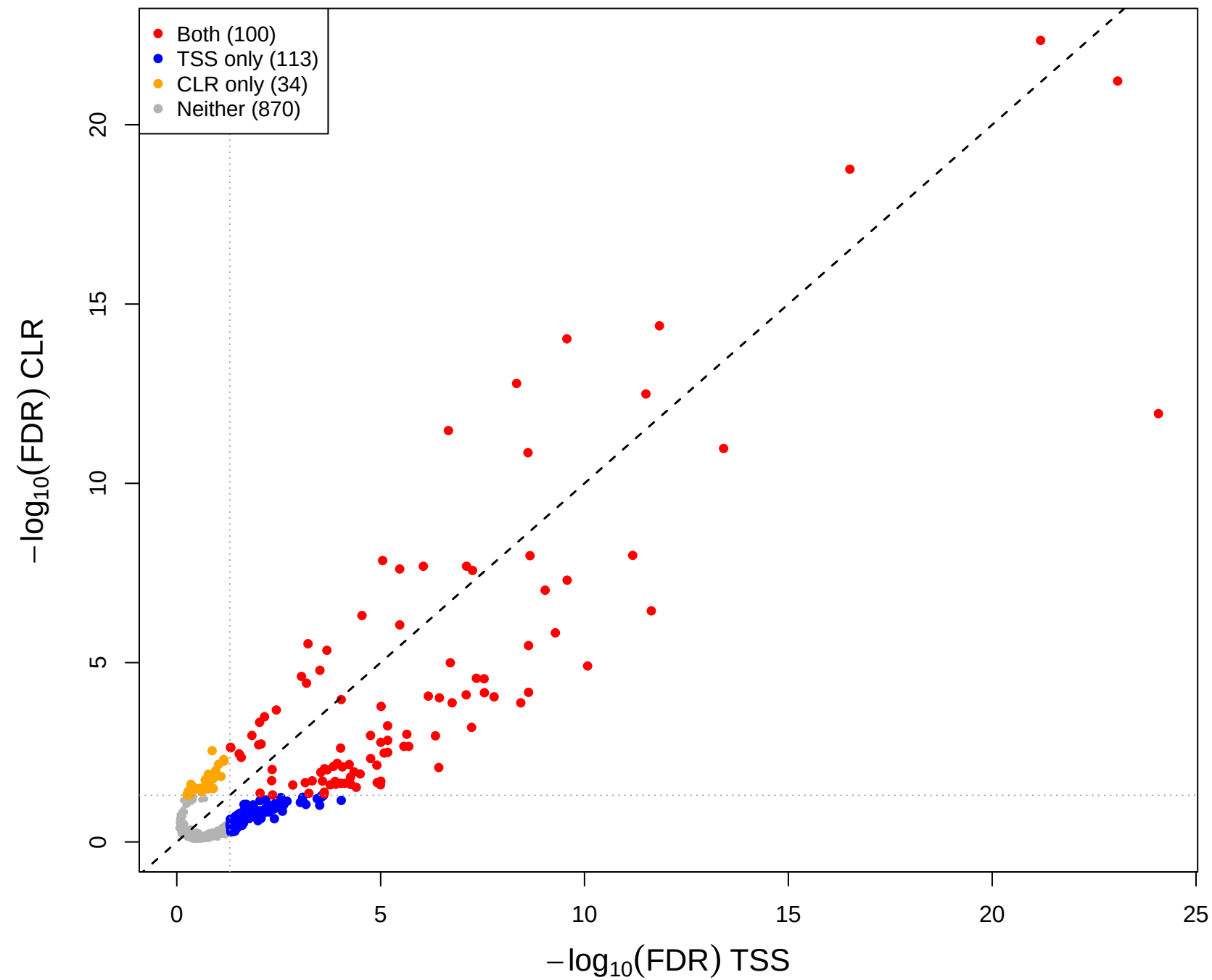
eld vs kin – CLR vs TSS(const=-0.9) (gamma = 0.5)
