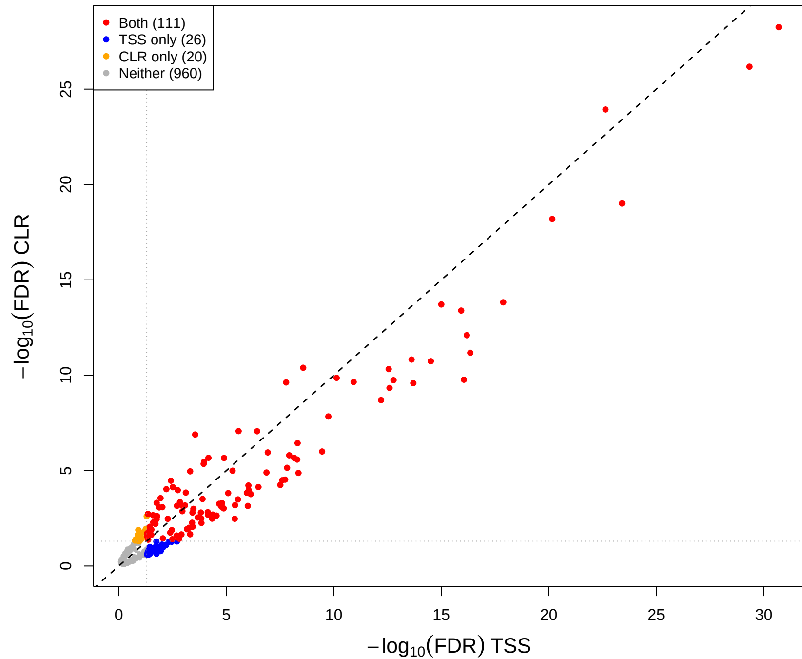
eld vs kin – CLR vs TSS(const=0.6) (gamma = 0.5)
