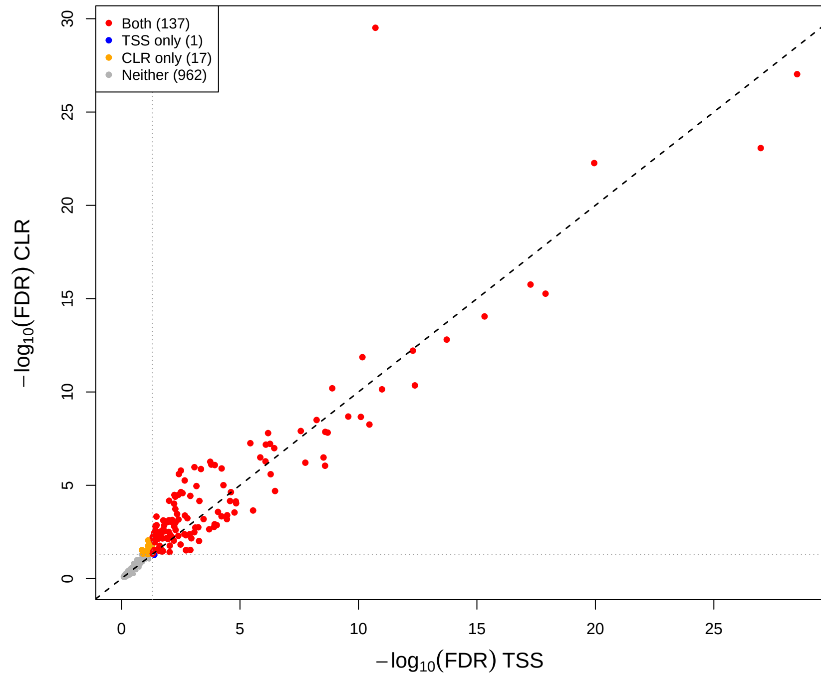
eld vs kin – CLR vs TSS(const=0) (gamma = 0.5)
