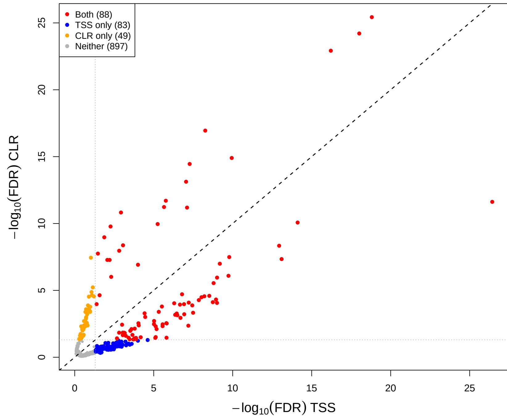
eld vs kin - CLR vs TSS(const=-1) (gamma = 0.5)
