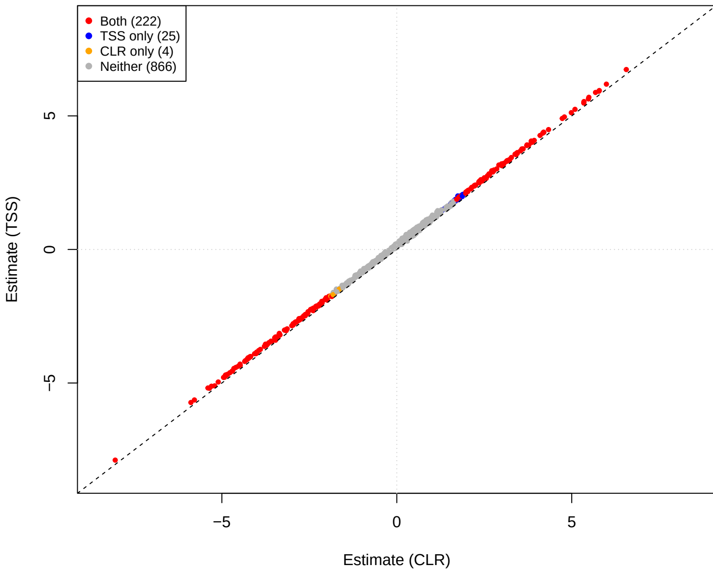
pup vs you [gamma = 0.5]
