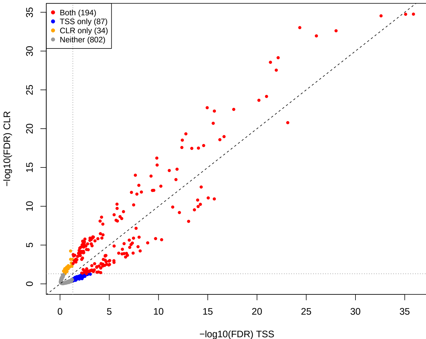
eld vs pup – CLR vs TSS (gamma = 0.3)
