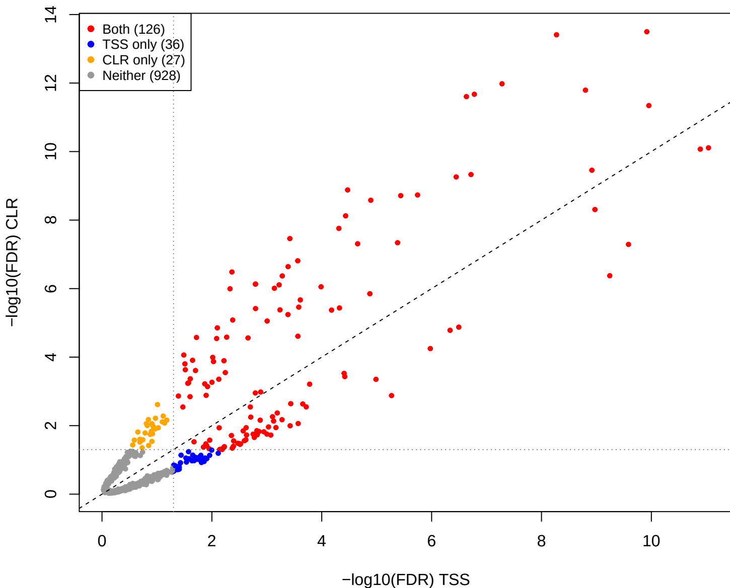
cent vs mage – CLR vs TSS (gamma = 0.3)
