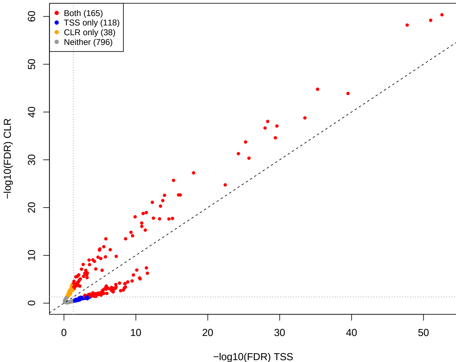
cent vs pup – CLR vs TSS (gamma = 0.5)
