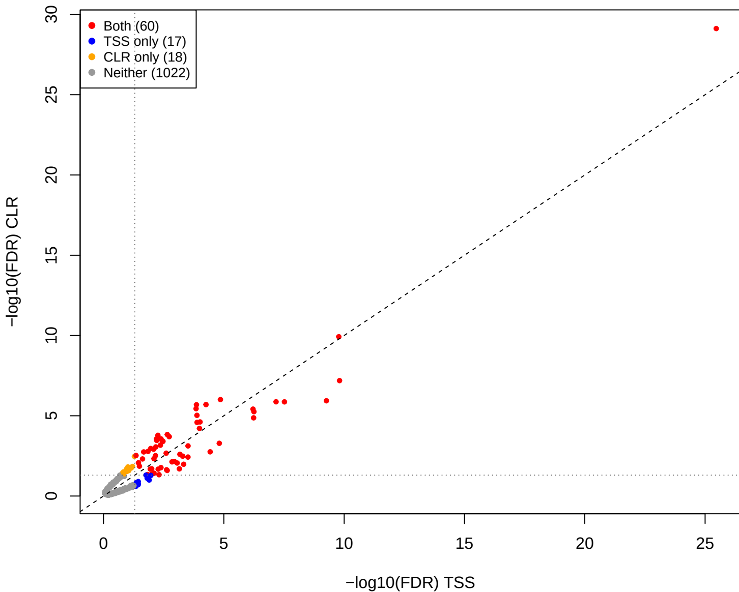
mage vs pup – CLR vs TSS (gamma = 0.5)
