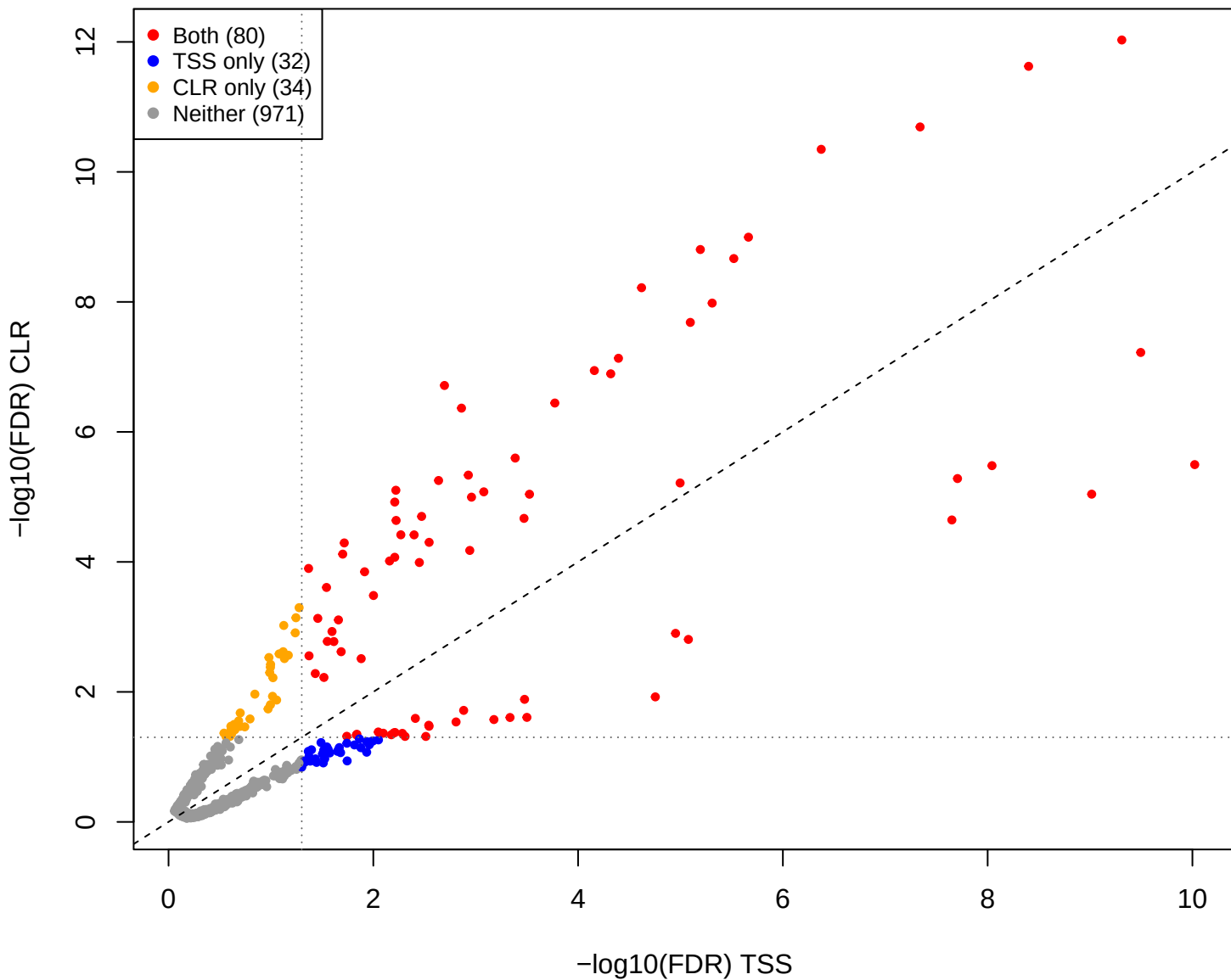
cent vs mage – CLR vs TSS (gamma = 0.5)
