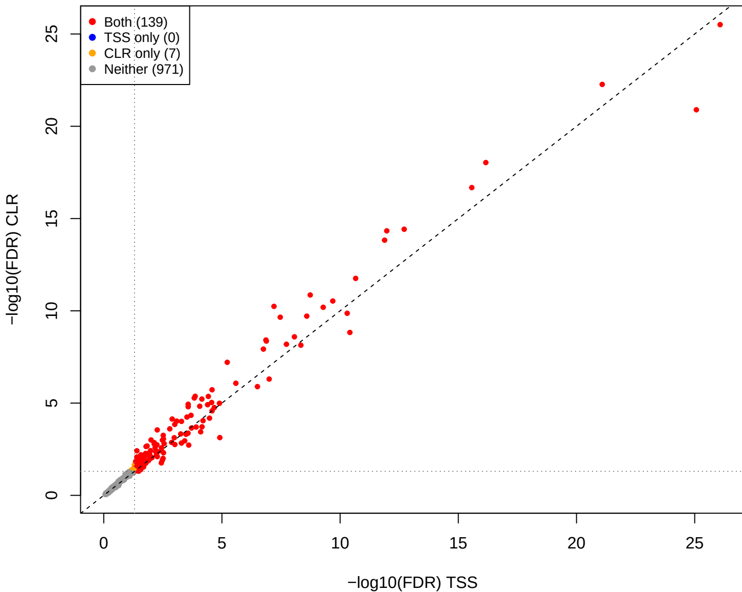
eld vs kin – CLR vs TSS (gamma = 0.5)
