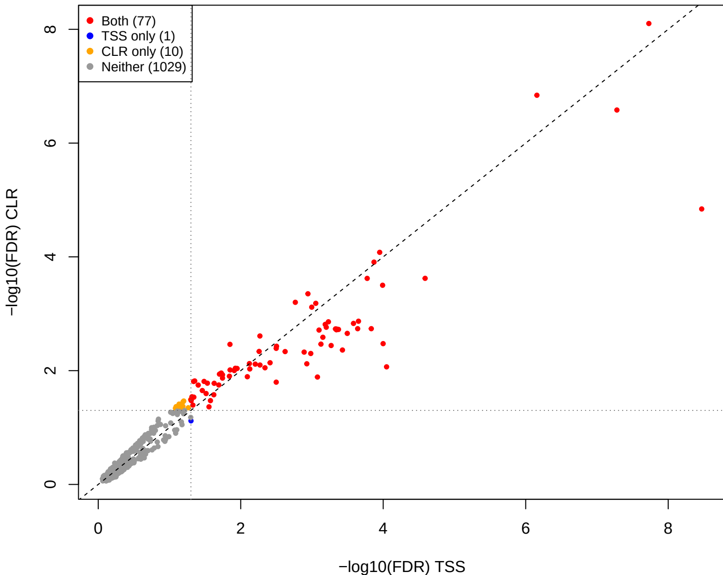
kin vs mid – CLR vs TSS (gamma = 0.5)
