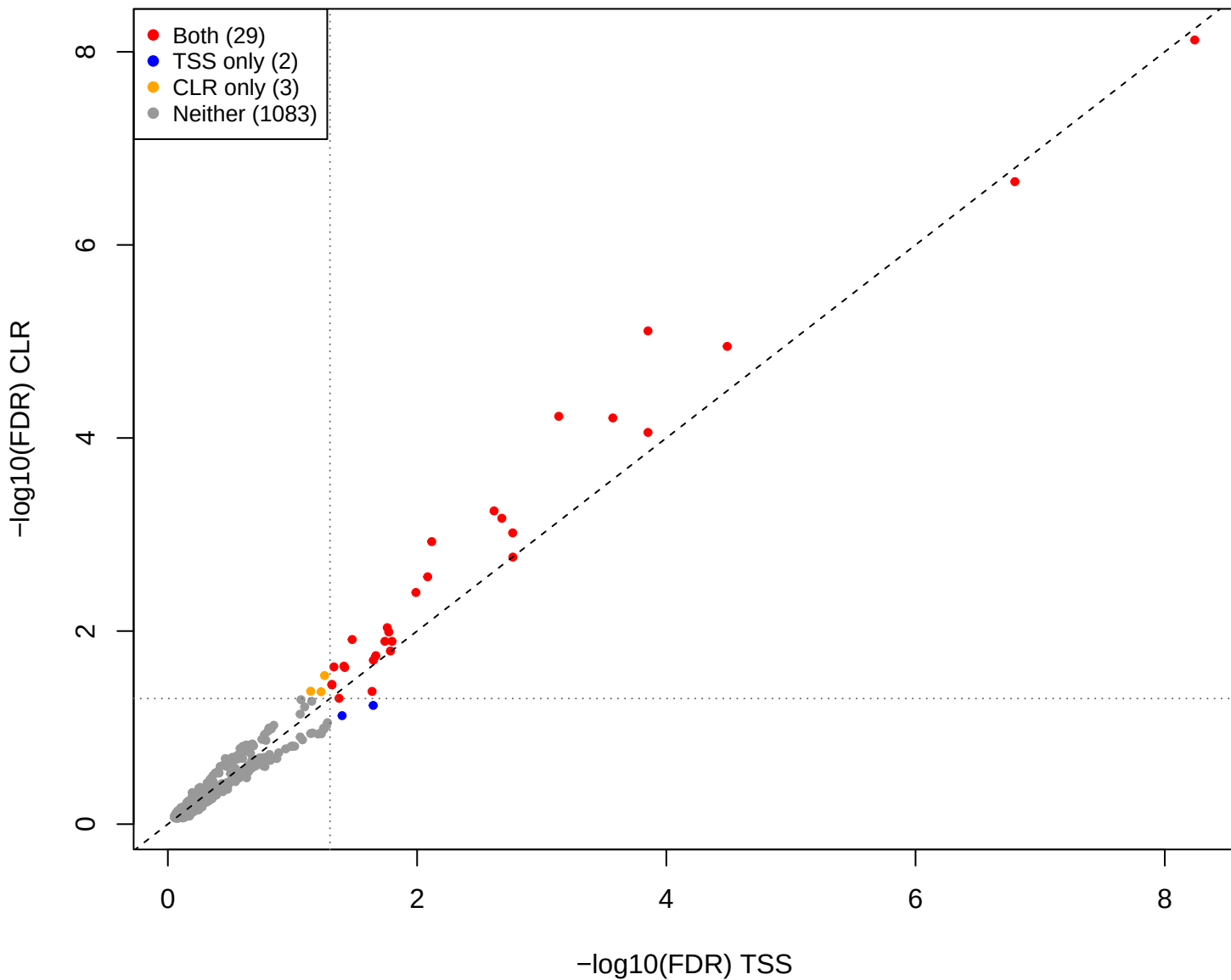
eld vs mage – CLR vs TSS (gamma = 0.5)
