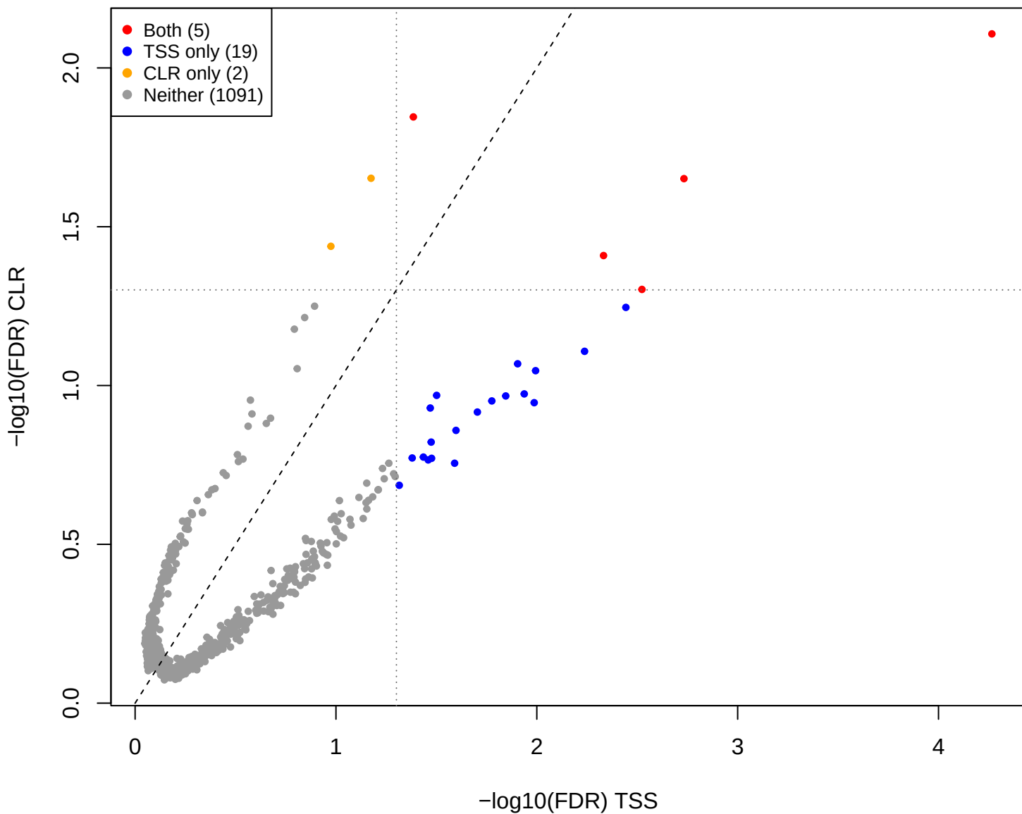
eld vs you – CLR vs TSS (gamma = 0.5)
