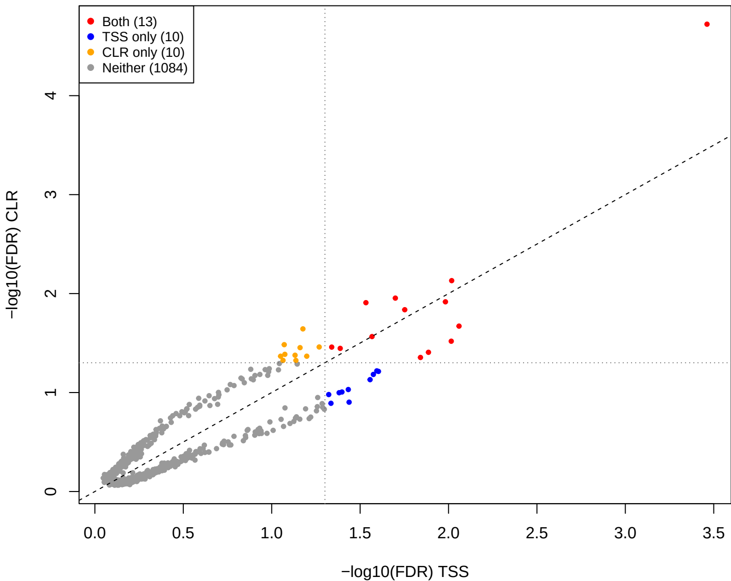
kin vs mage – CLR vs TSS (gamma = 0.5)
