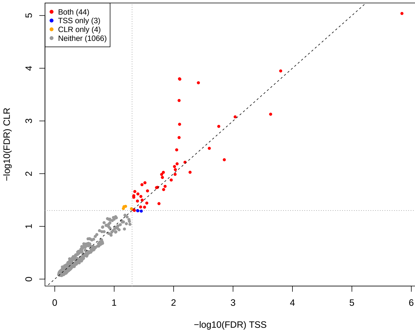
cent vs eld – CLR vs TSS (gamma = 0.5)
