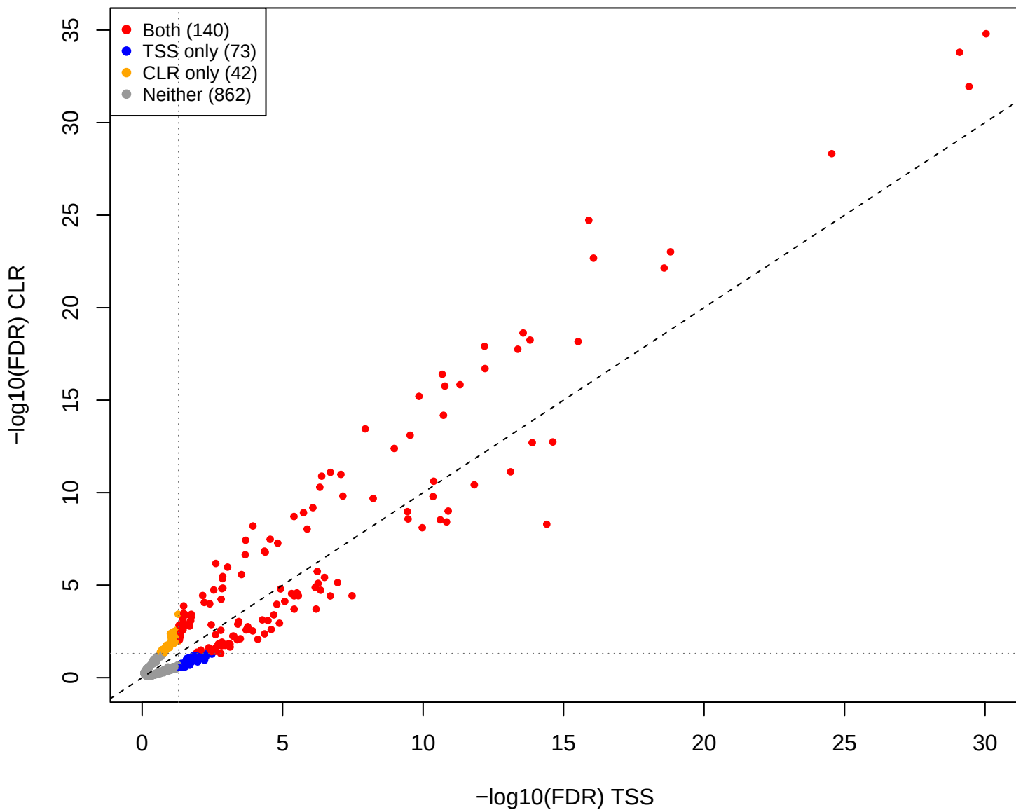
eld vs pup – CLR vs TSS (gamma = 0.5)
