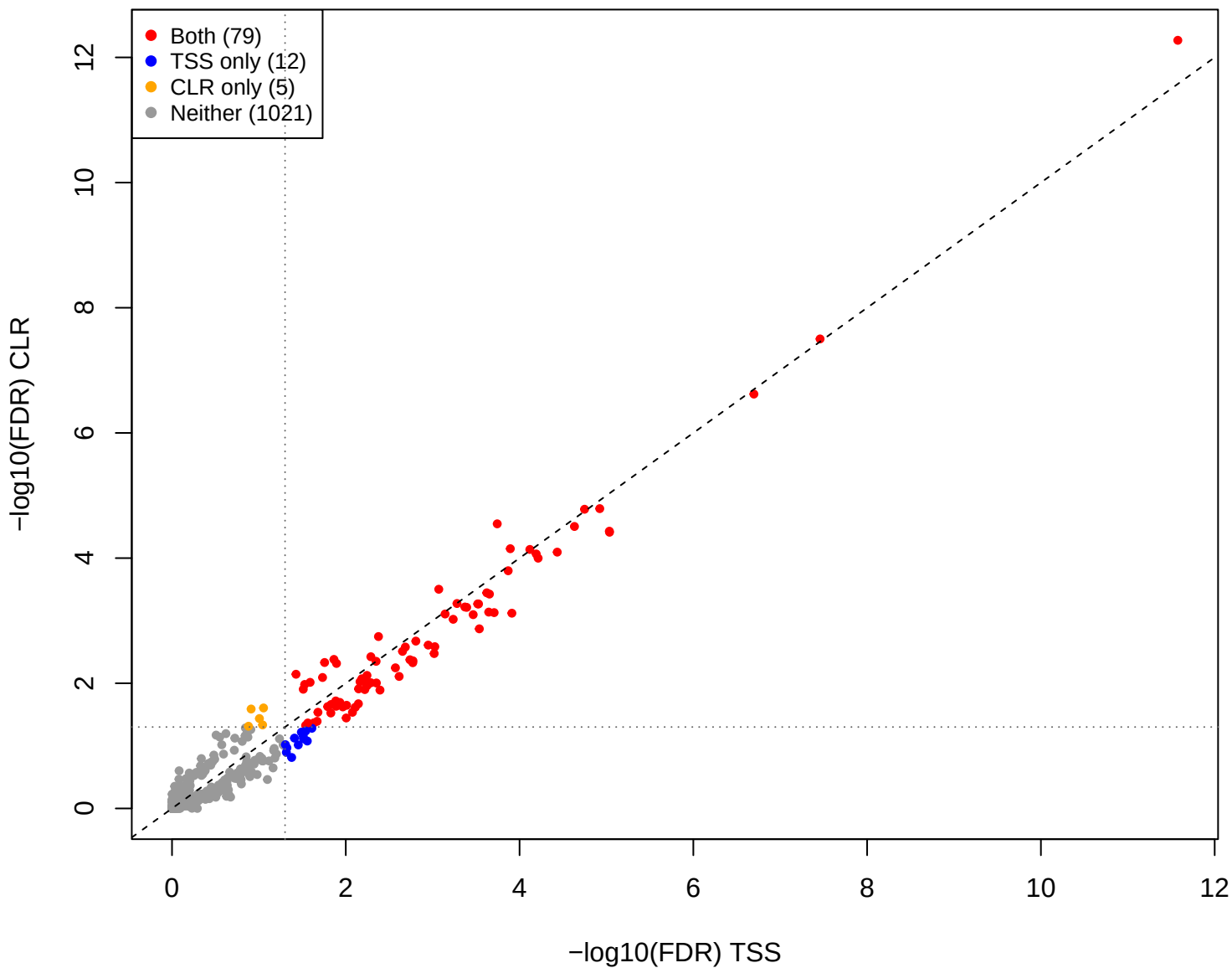
mage vs mid – CLR vs TSS (gamma = 1e-5)
