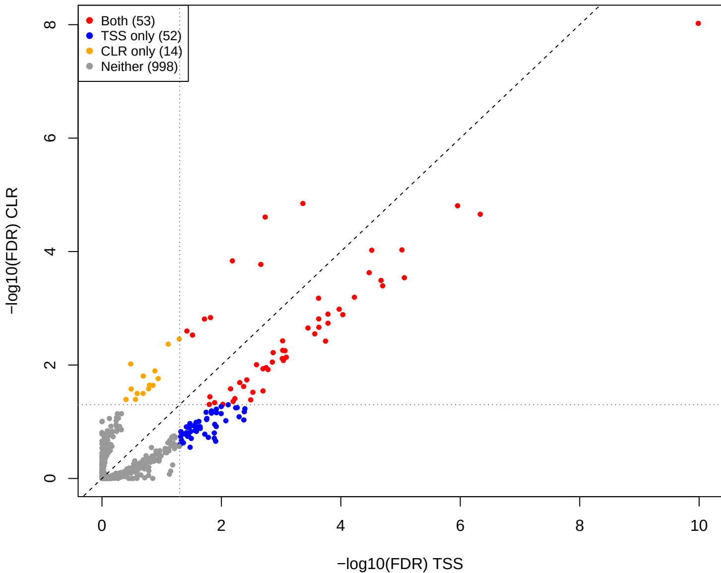
eld vs you – CLR vs TSS (gamma = 1e-5)
