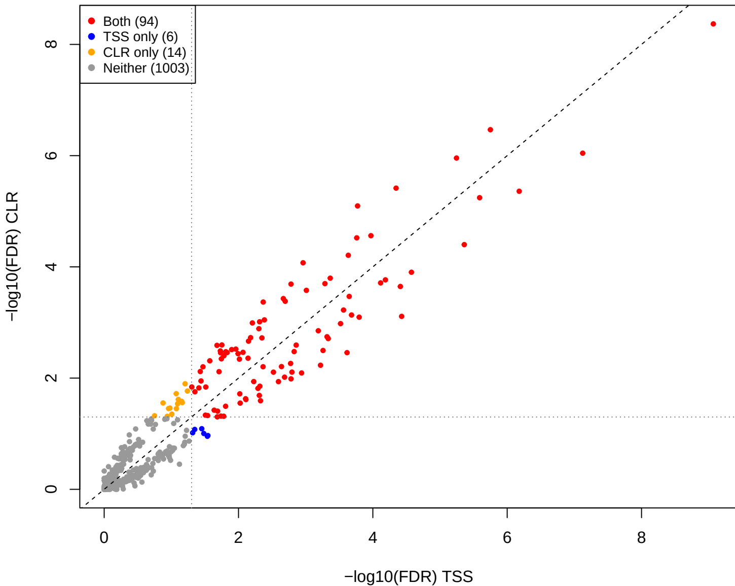
kin vs mage – CLR vs TSS (gamma = 1e-5)
