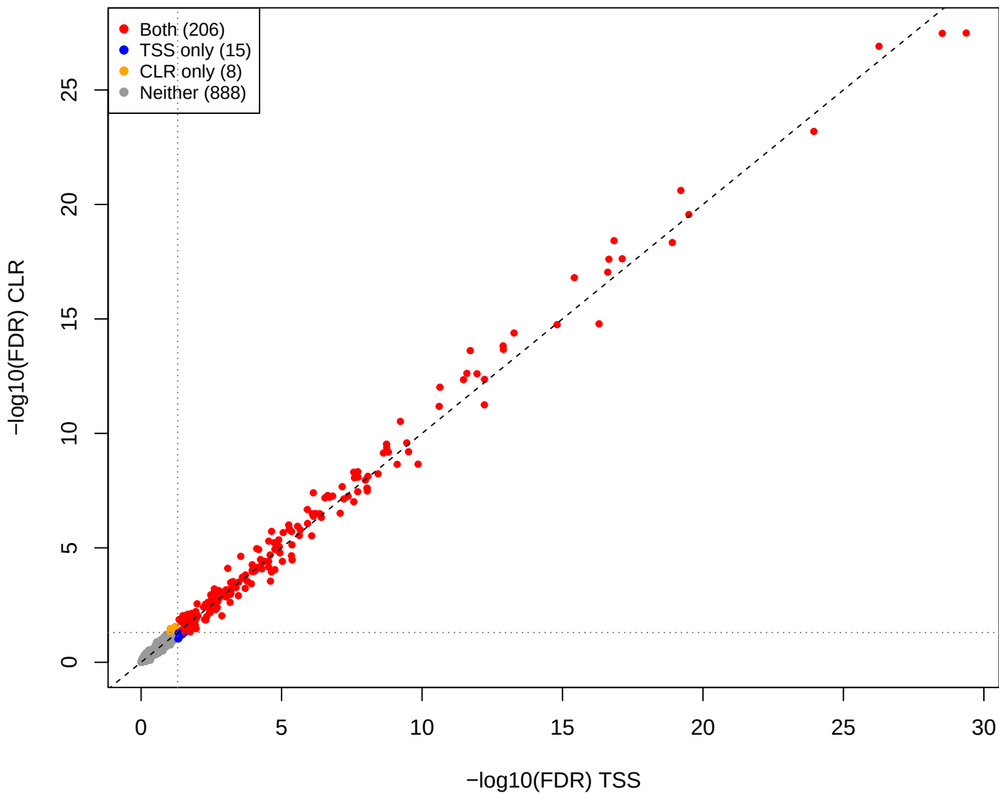
eld vs kin – CLR vs TSS (gamma = 1e-5)
