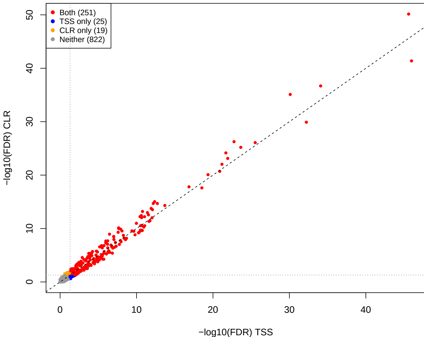
cent vs kin – CLR vs TSS (gamma = 1e-5)
