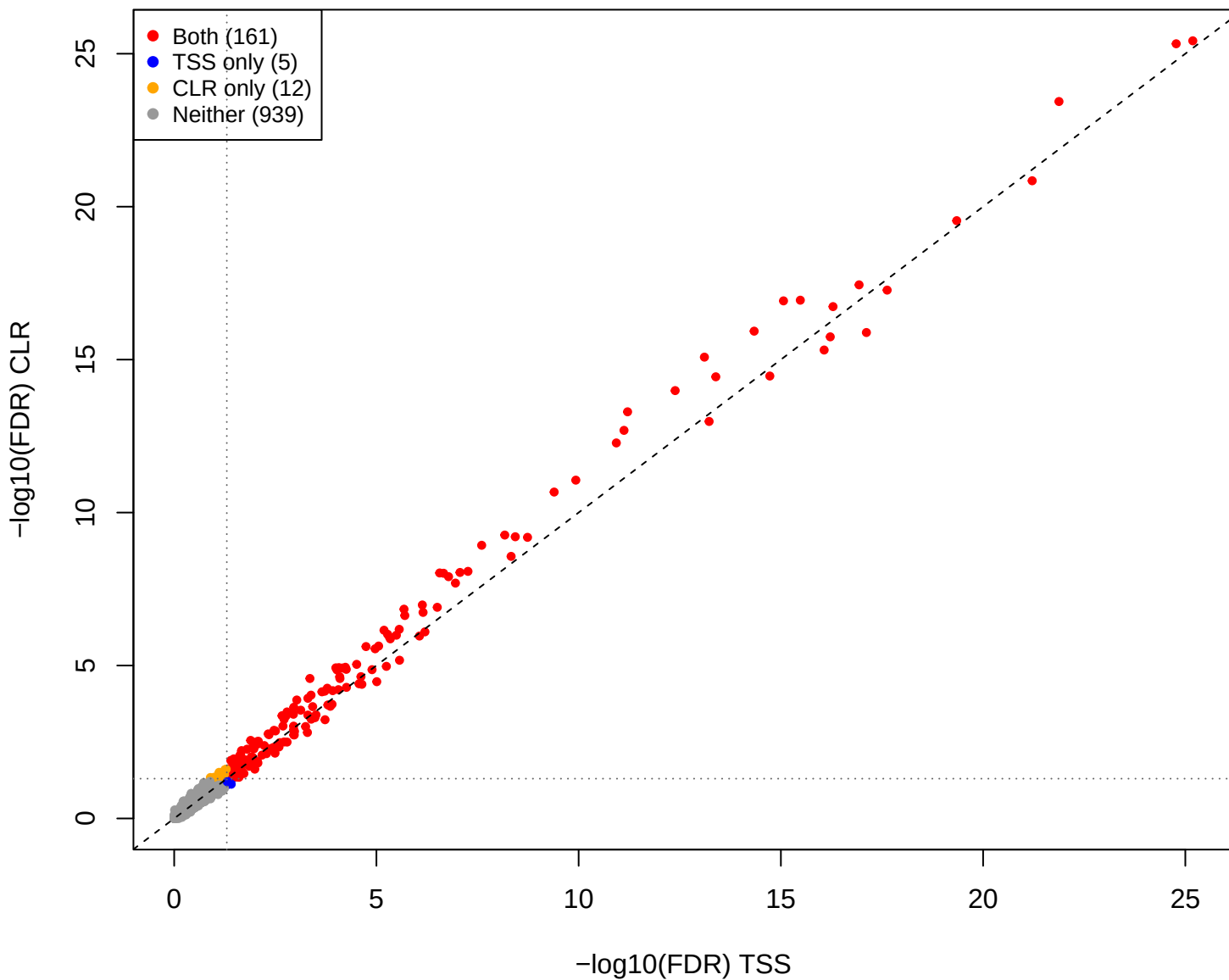
eld vs mid – CLR vs TSS (gamma = 1e-5)
