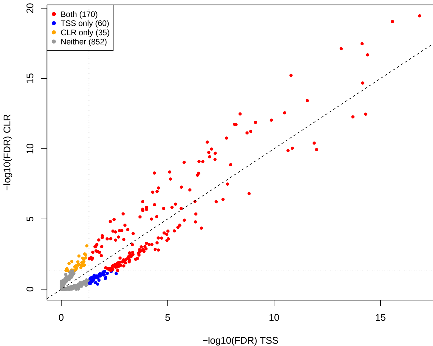
cent vs mage – CLR vs TSS (gamma = 1e-5)
