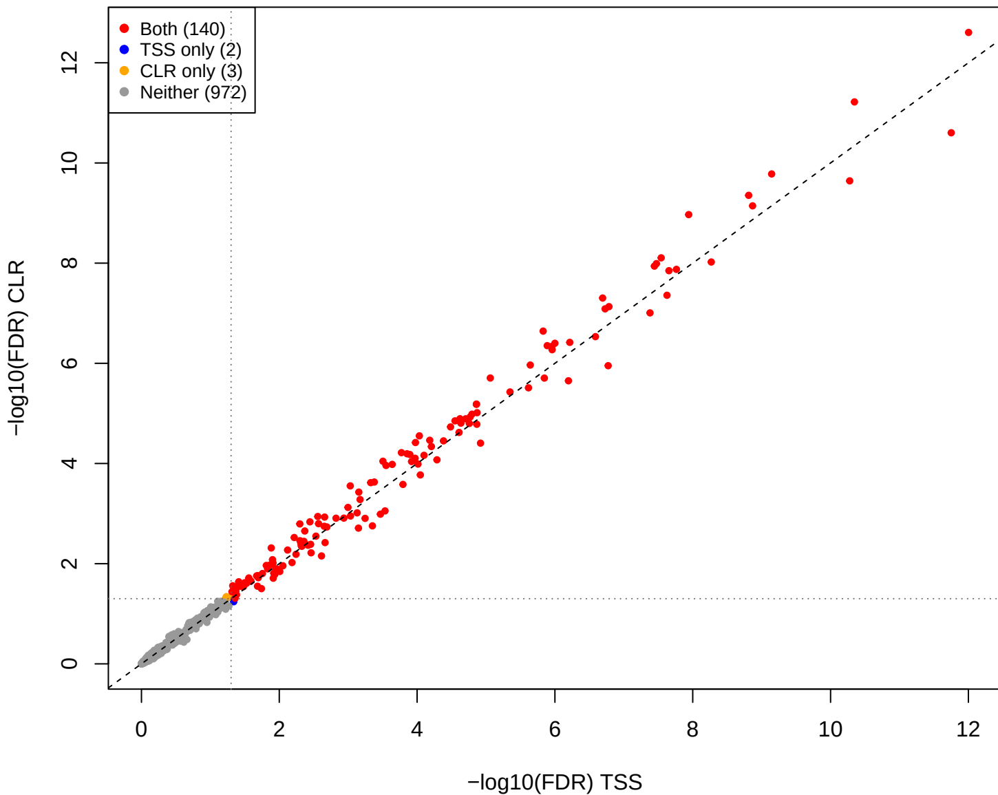
kin vs mid – CLR vs TSS (gamma = 1e-5)
