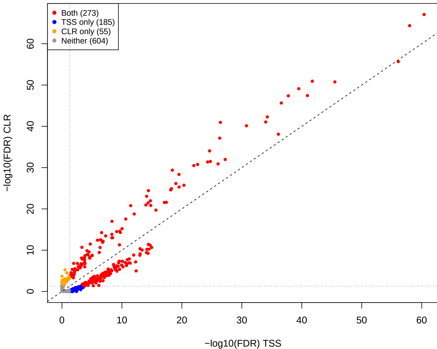
cent vs pup – CLR vs TSS (gamma = 1e-5)
