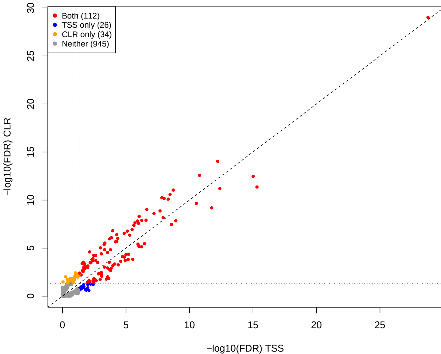
mage vs pup – CLR vs TSS (gamma = 1e-5)
