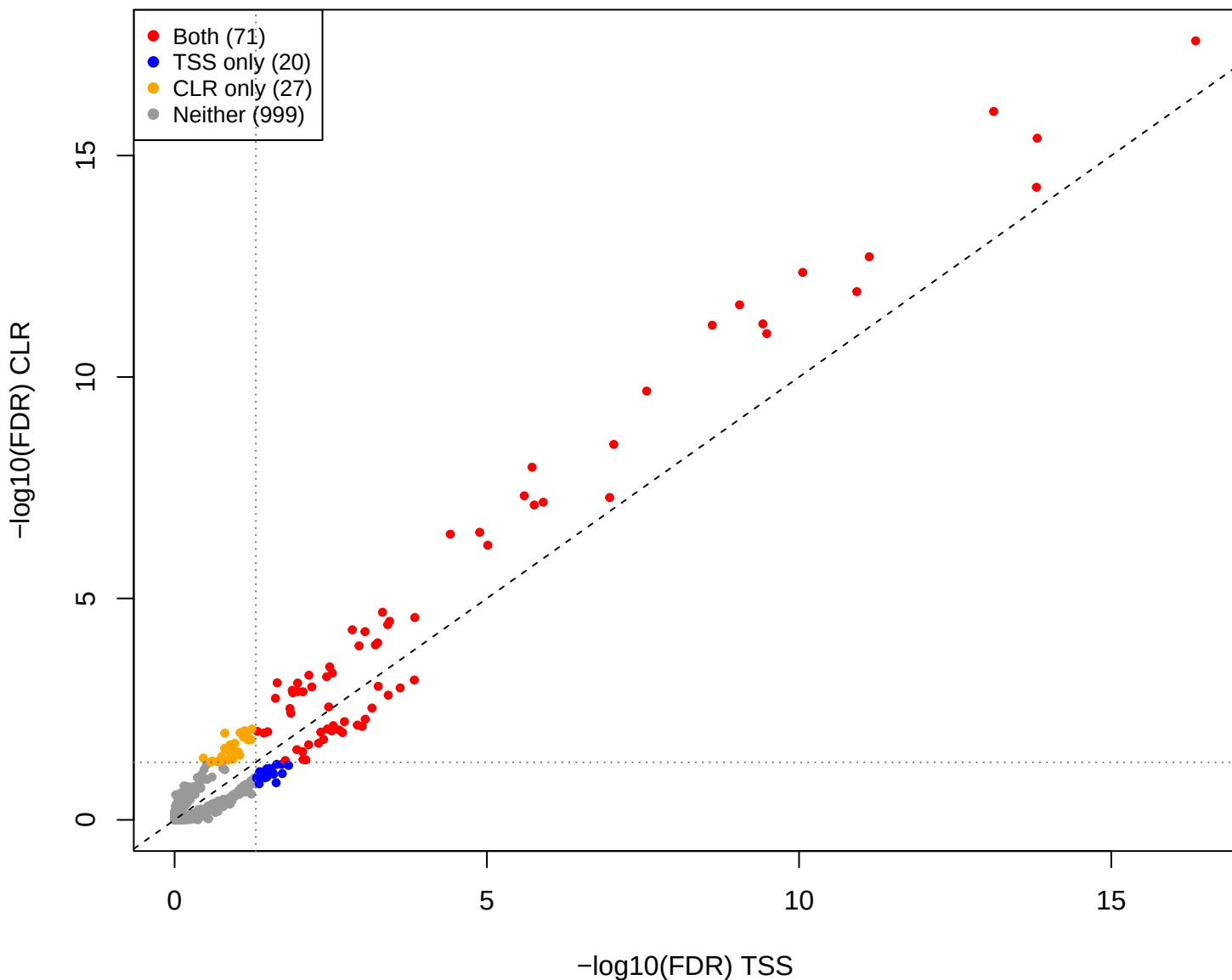
eld vs mage – CLR vs TSS (gamma = 1e-5)
