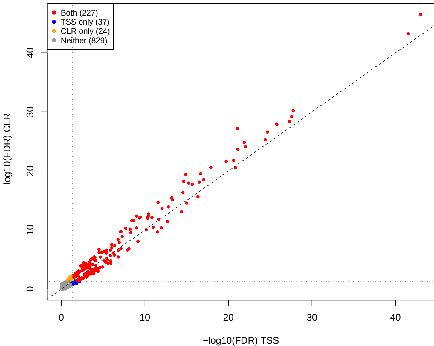
cent vs mid – CLR vs TSS (gamma = 1e-5)
