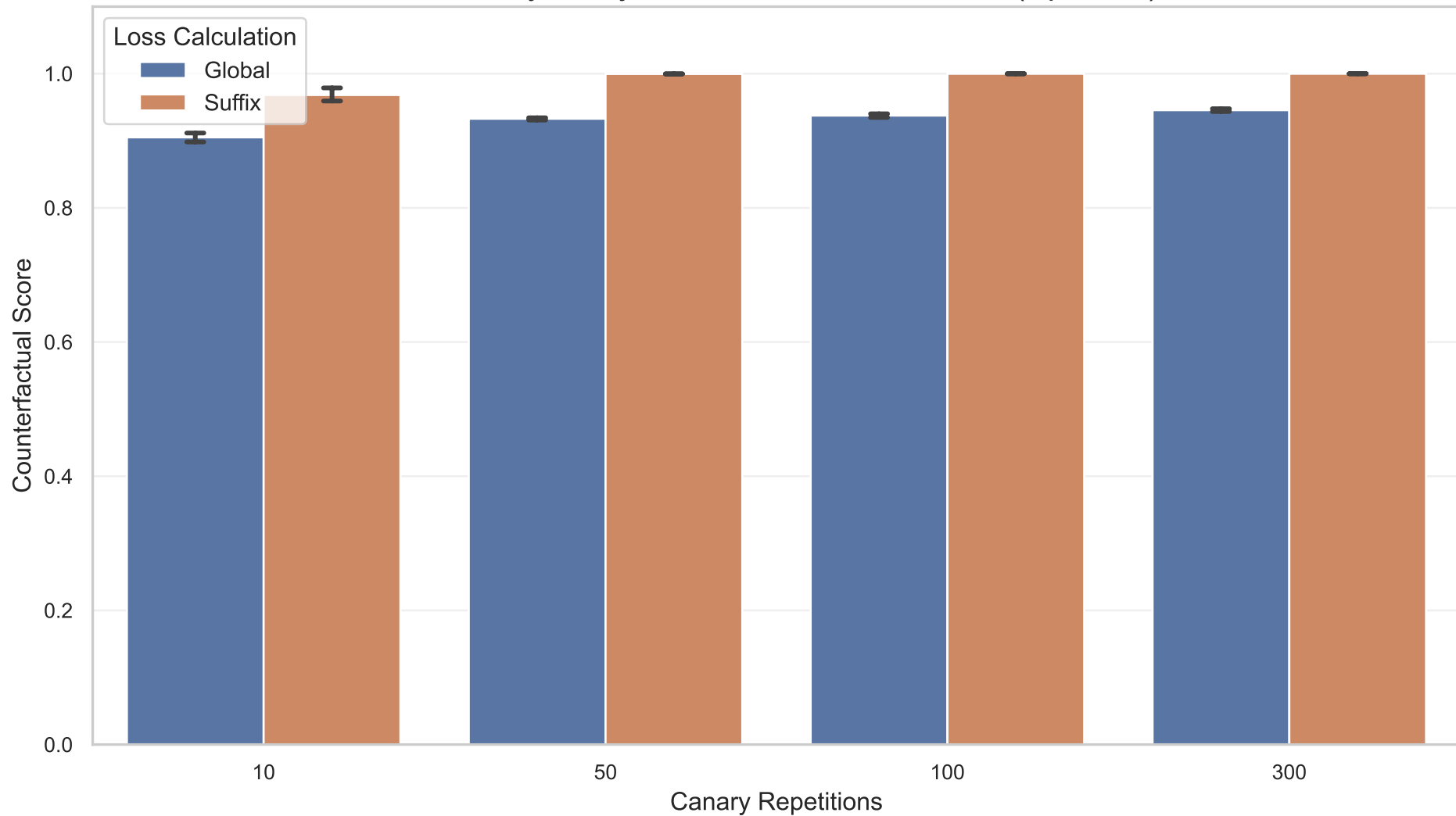
Sensitivity Analysis: Global vs Suffix Loss (Epoch 9)
