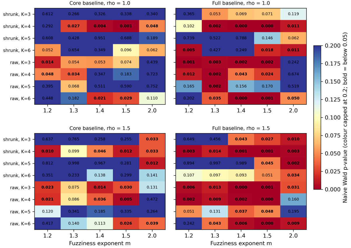
Figure 7.1: Conventional Wald p -values across the specification grid
