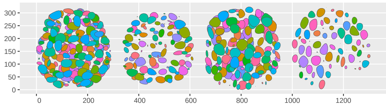
adhd200_400 subcortical atlas
