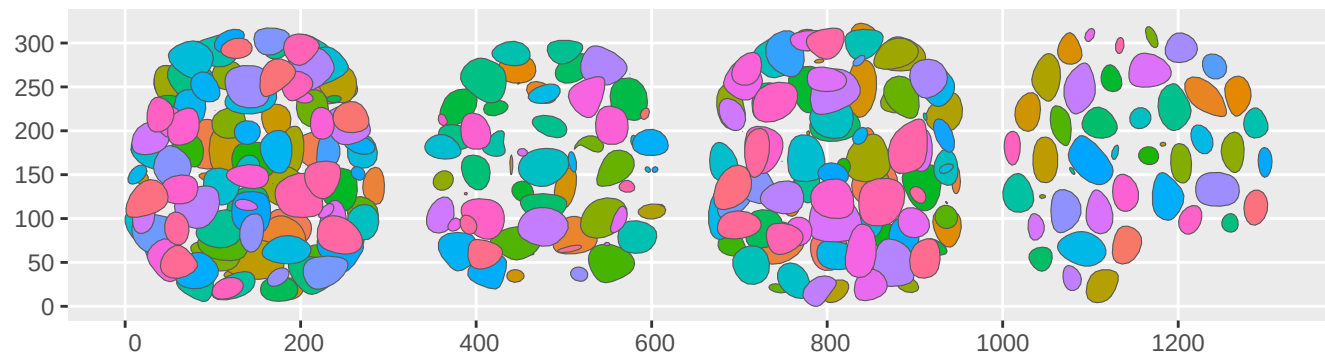
adhd200_200 subcortical atlas
