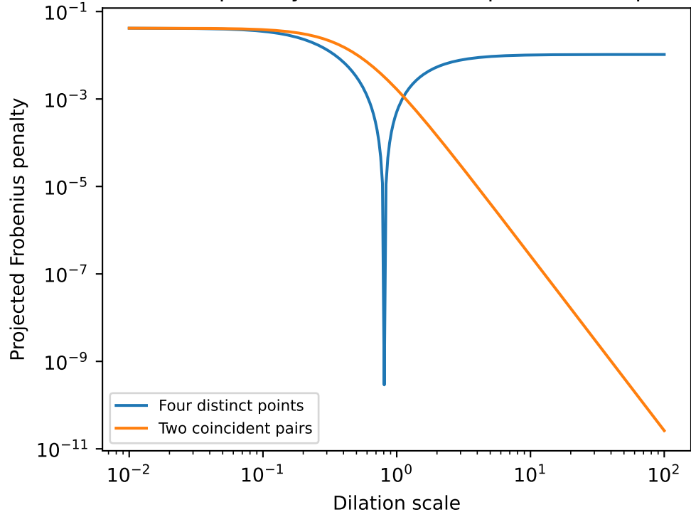
A trace penalty alone does not prevent escape
