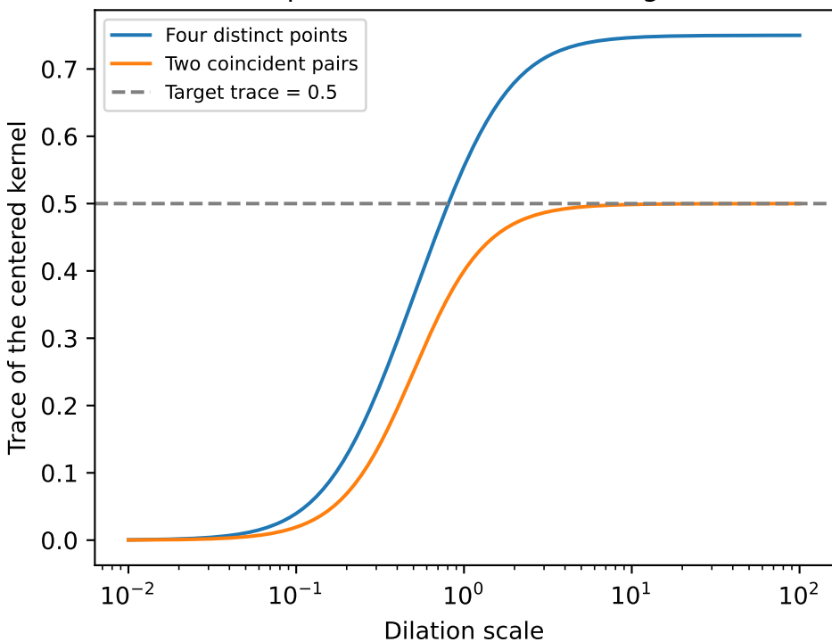
Trace depends on scale and configuration
