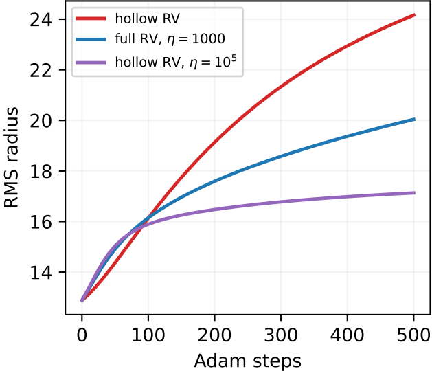
Coordinate-space evolution
