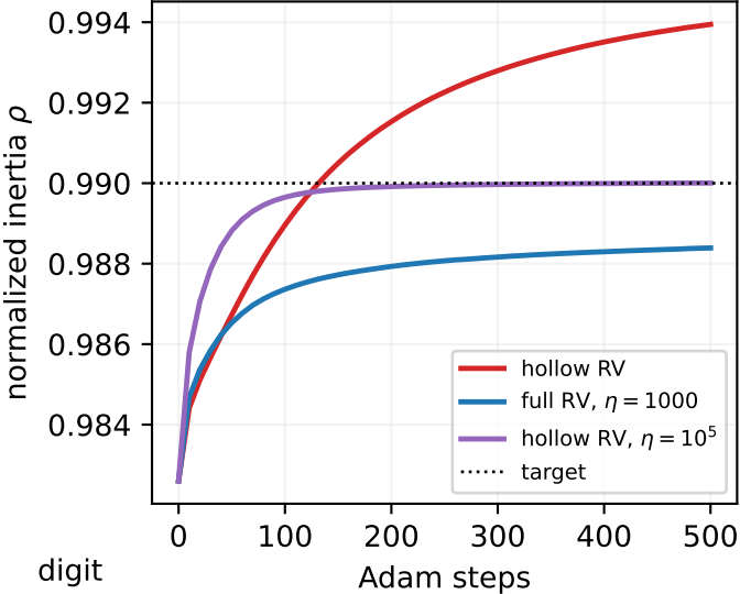
Kernel-space evolution
