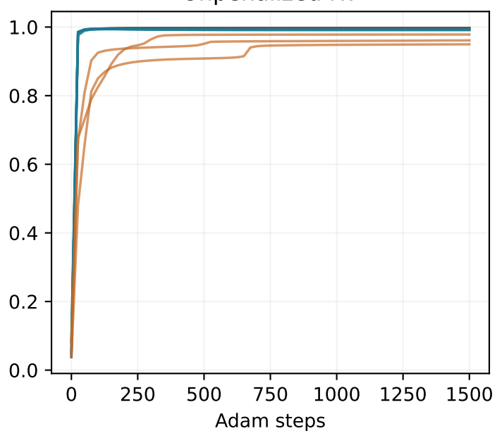
Unpenalized RV
