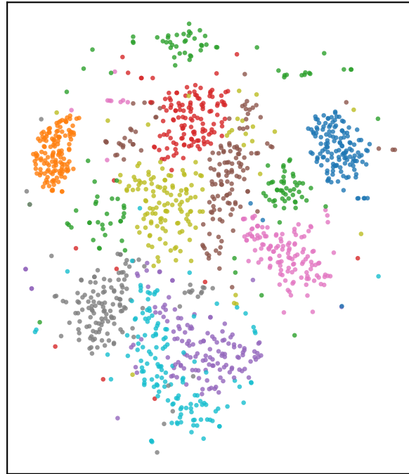
Supervised dial: t-SNE ( \beta=0 ) \rightarrow classkernel ( \beta=1 ), train embeddings
