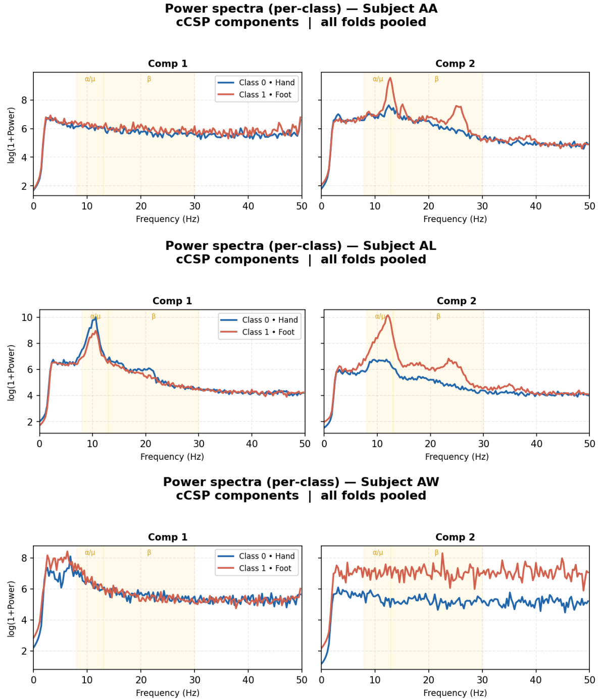
Figure B. Per-subject full power spectra for fixed-config cSP (1 feature) with mu and beta bands annotated.
