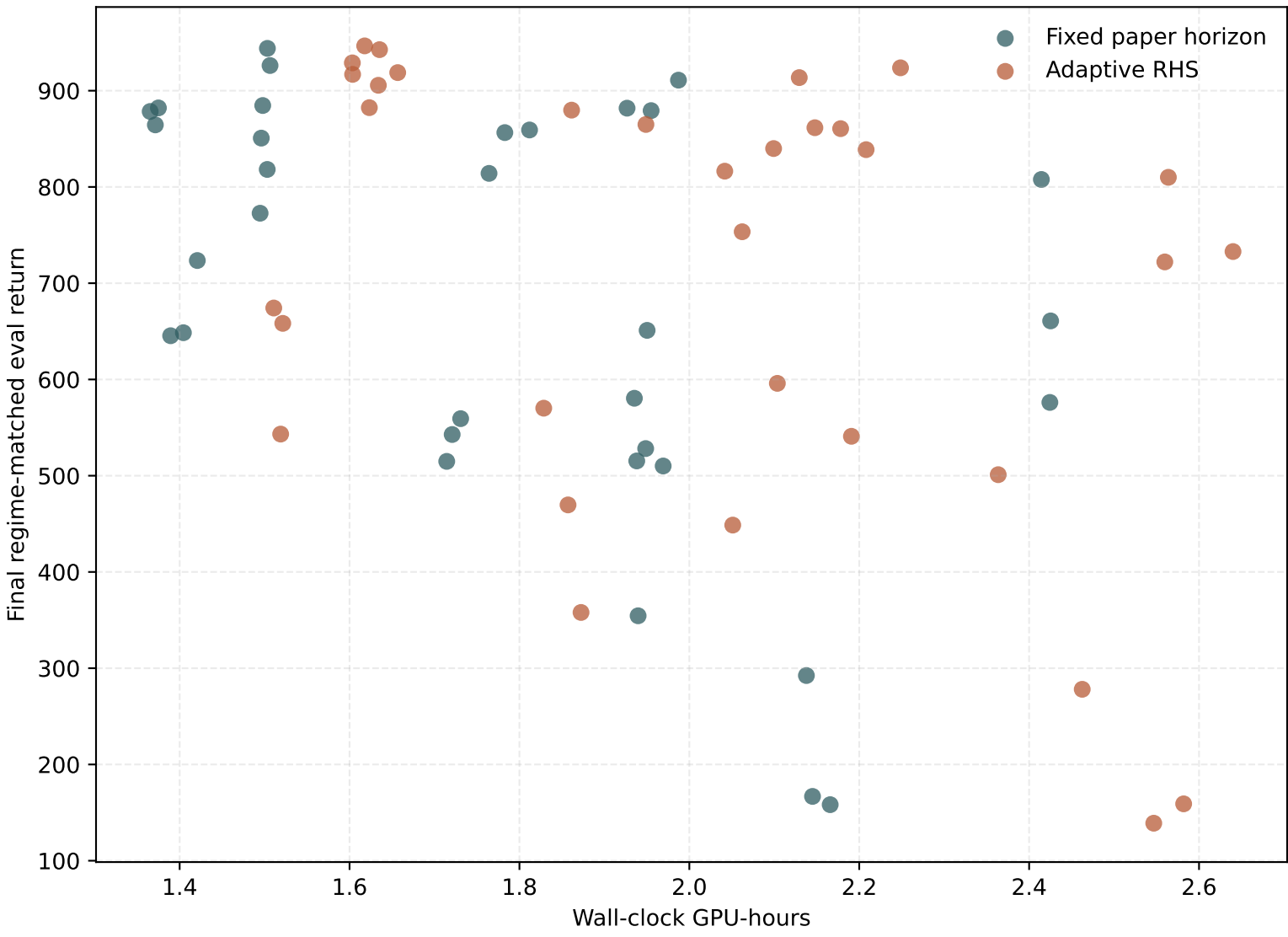
Compute-performance tradeoff
