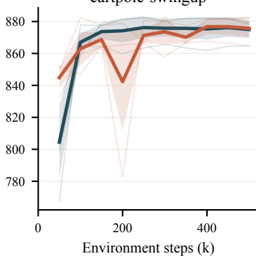
cartpole-swingup
