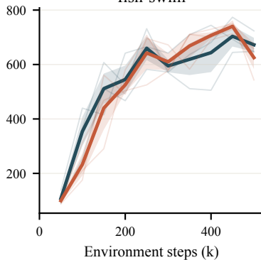
fish-swim
