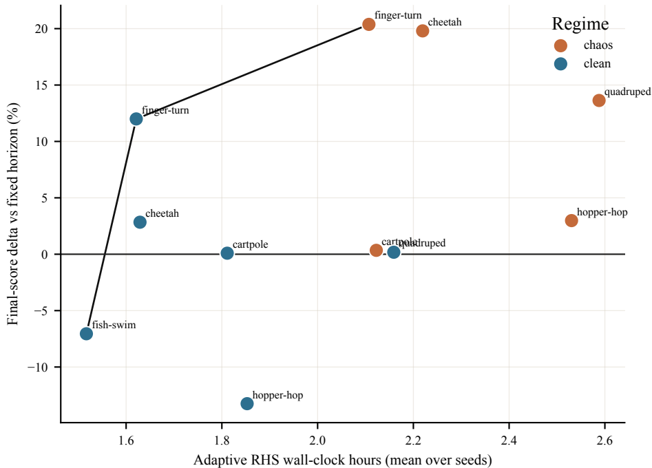
Compute-performance Pareto view
