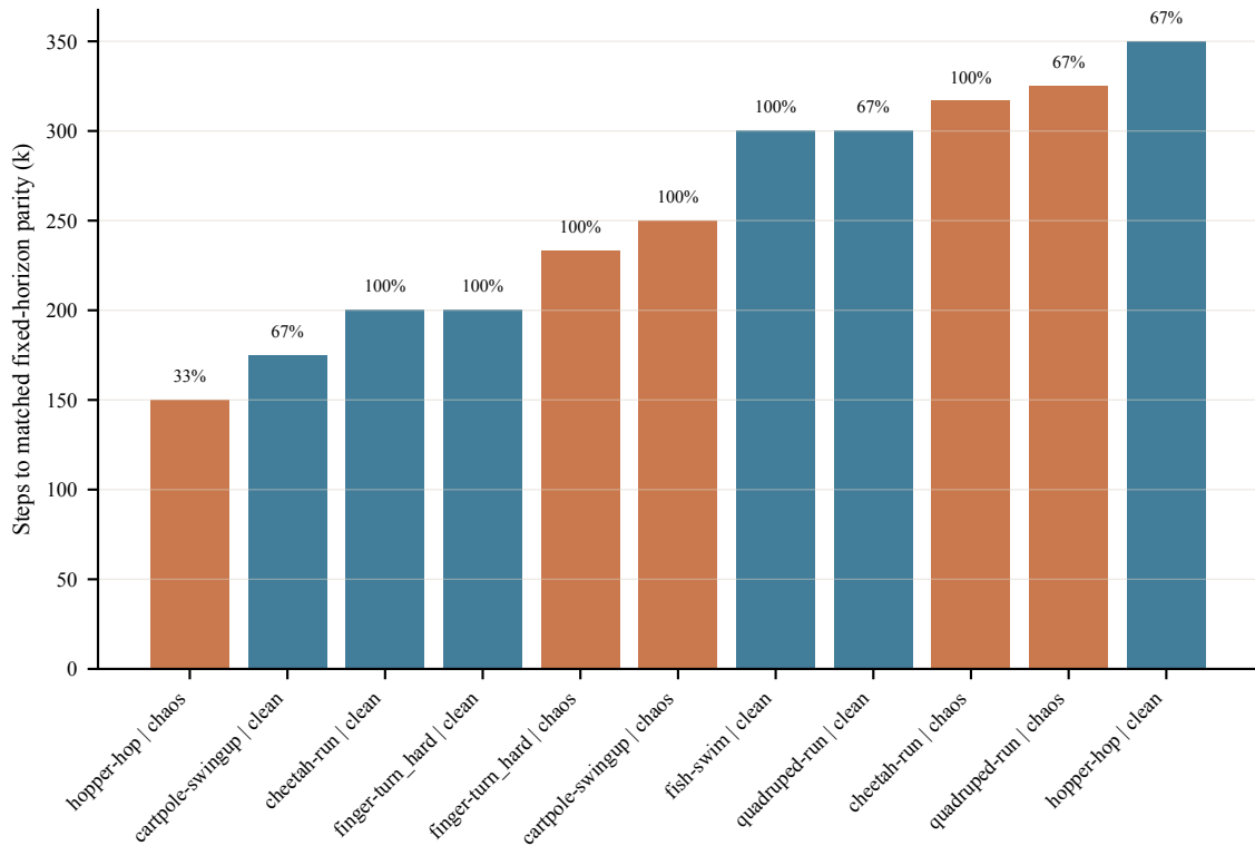
Sample efficiency: reaching matched baseline final score
