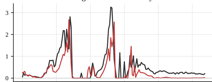
Right Knee Loaded Flexion
