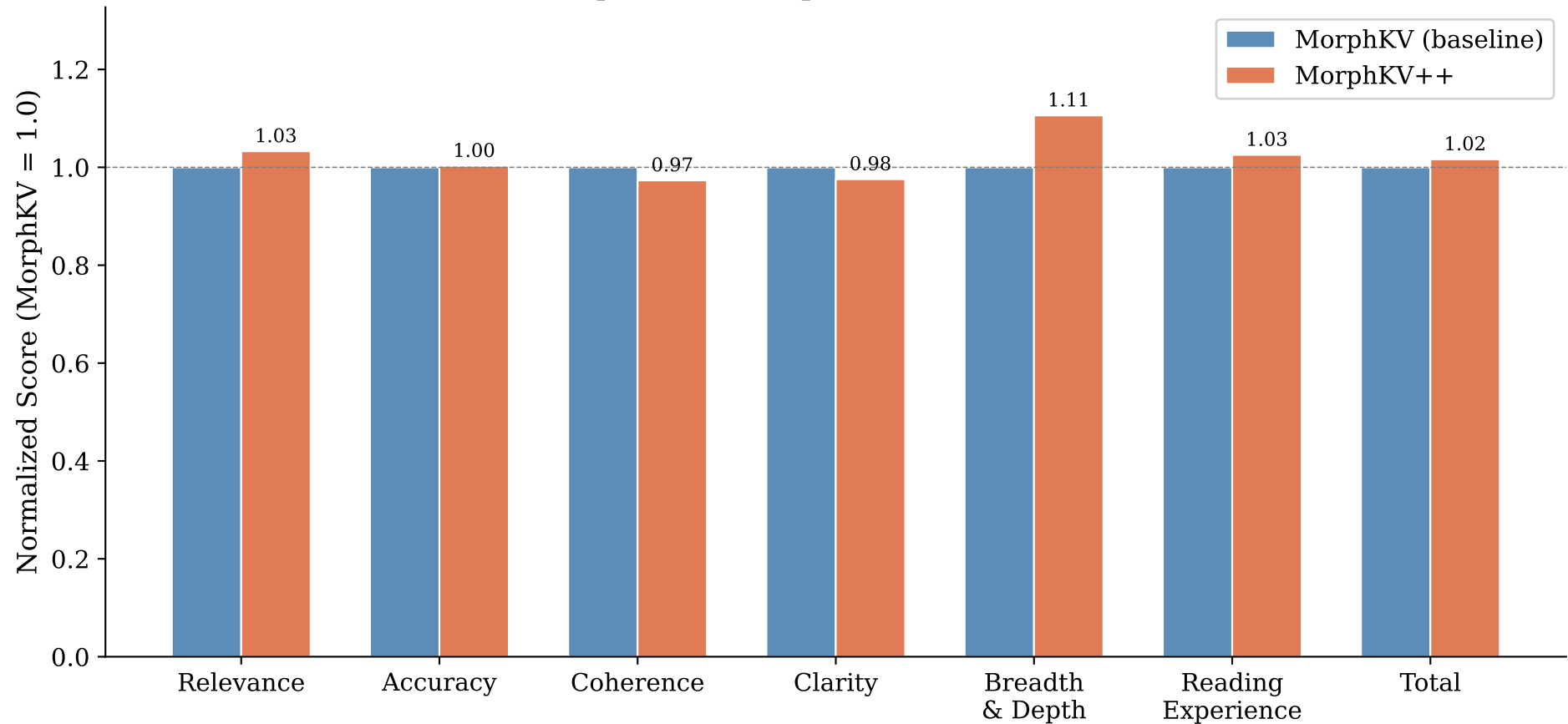
MorphKV vs MorphKV++ — Qwen-2.5
