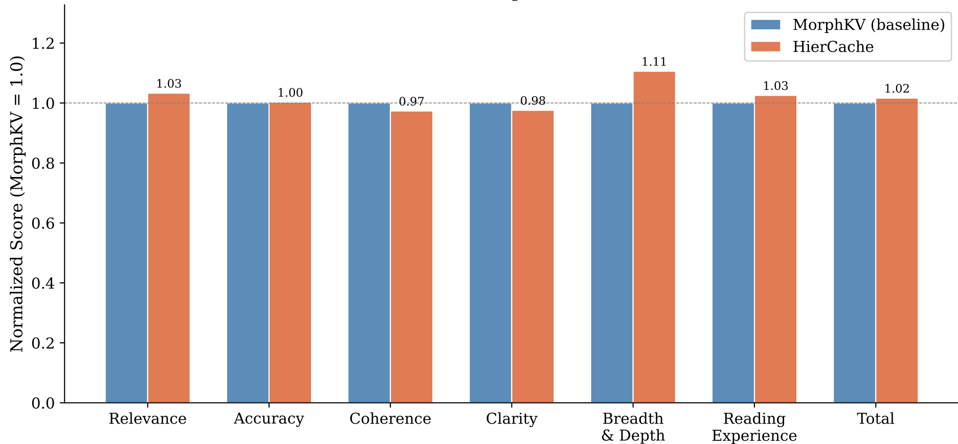
HierCache vs MorphKV — Qwen-2.5
