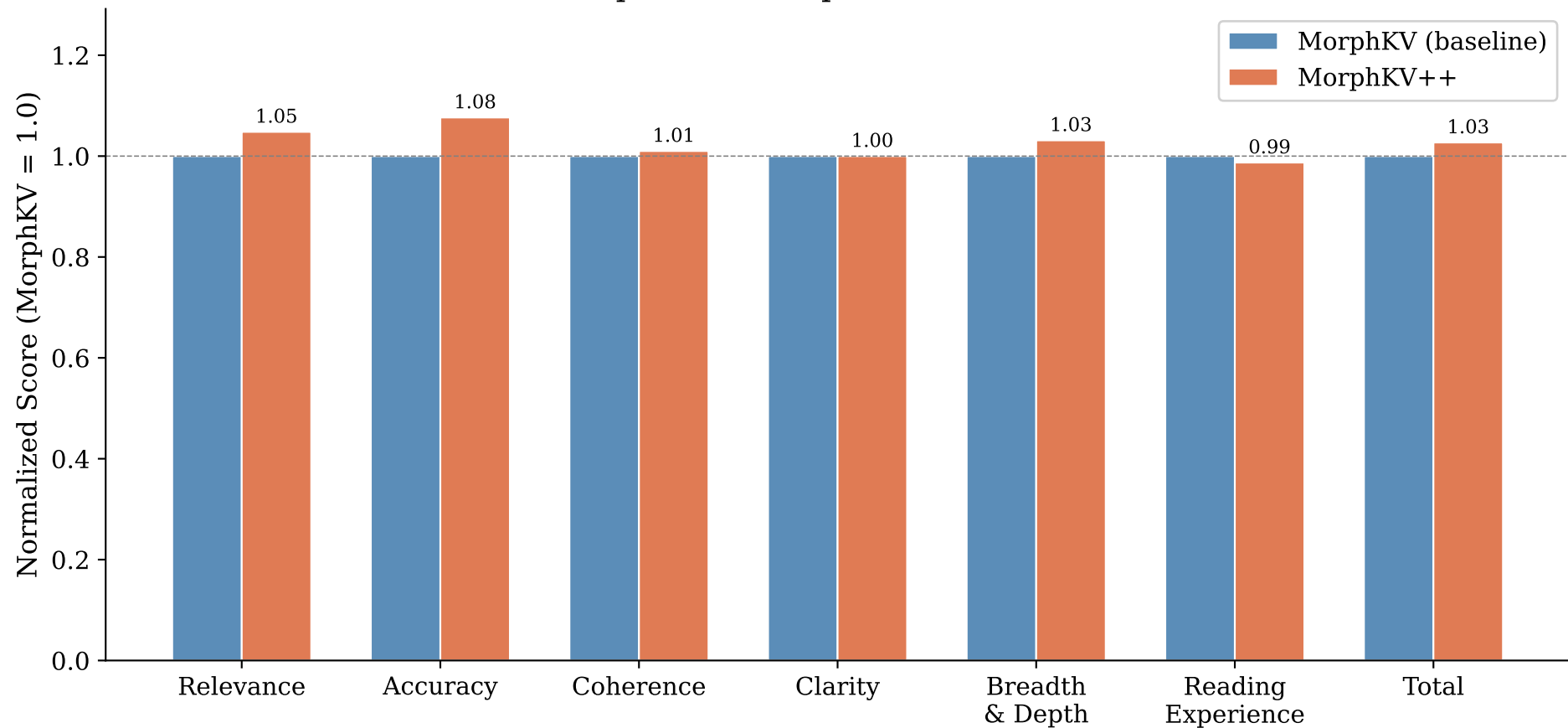
MorphKV vs MorphKV++ — Mistral
