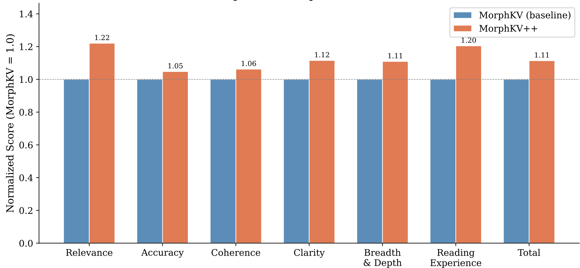
MorphKV vs MorphKV++ — Phi-4
