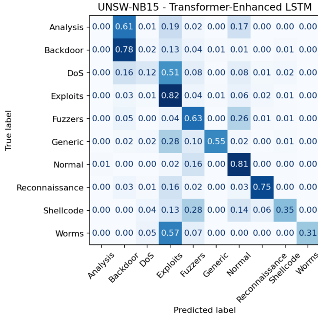
Fig. 7. Confusion Matrix for UNSW-NB15.
