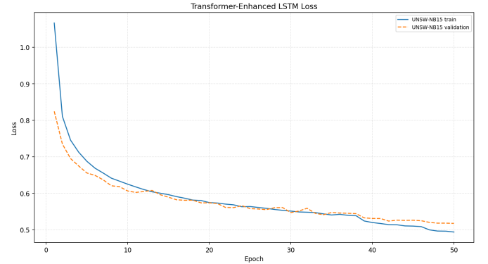
Fig. 6. Training and Validation Loss Curve for UNSW-NB15.
