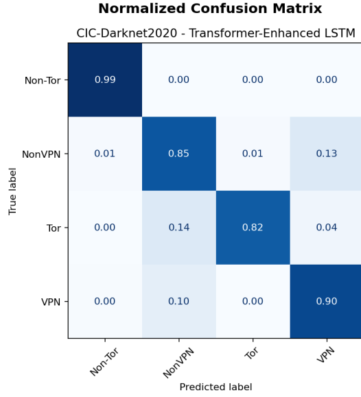
Fig. 4. Confusion Matrix for CIC-Darknet2020.
