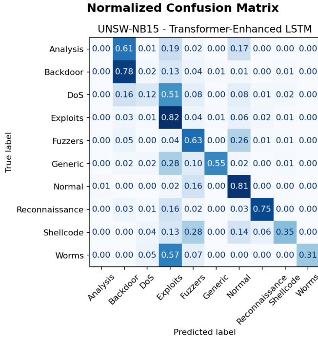
Fig. 7. Confusion Matrix for UNSW-NB15.
