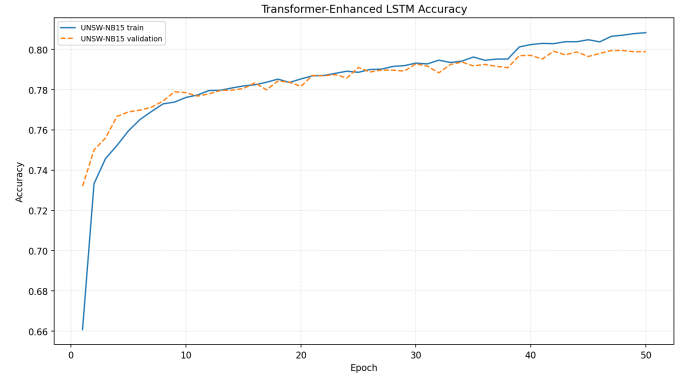
Fig. 5. Training and Validation Accuracy Curve for UNSW-NB15.
