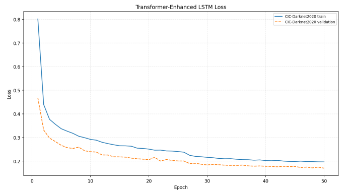
Fig. 3. Training and Validation Loss Curve of CIC-Darknet2020.
