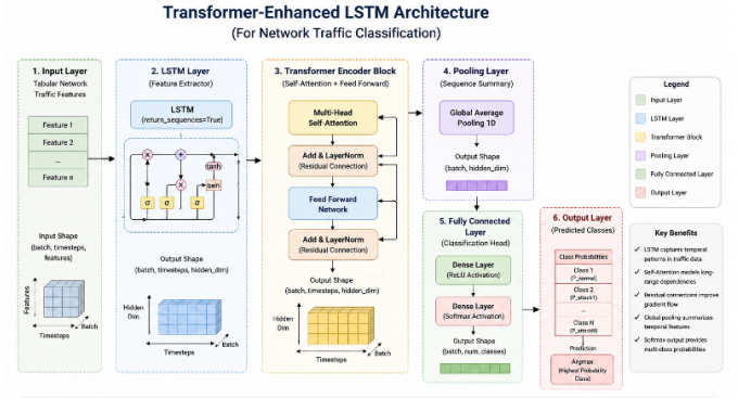
Fig. 1. Proposed transformer-enhanced LSTM architecture.
