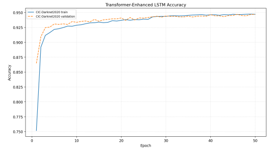
Fig. 2. Training and Validation Accuracy Curve of CIC-Darknet2020.
