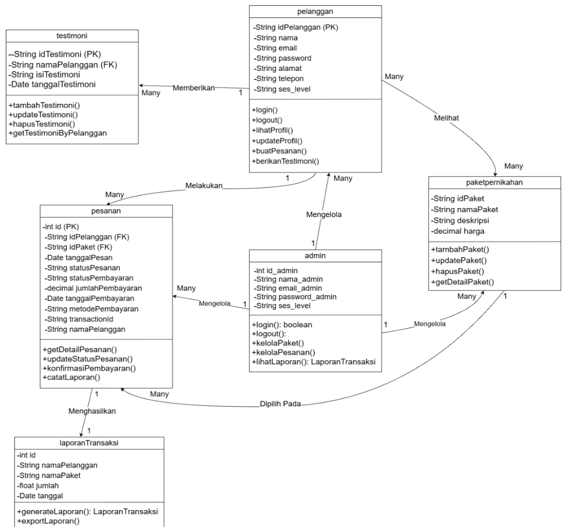
Gambar 3. 12 Class Diagram
