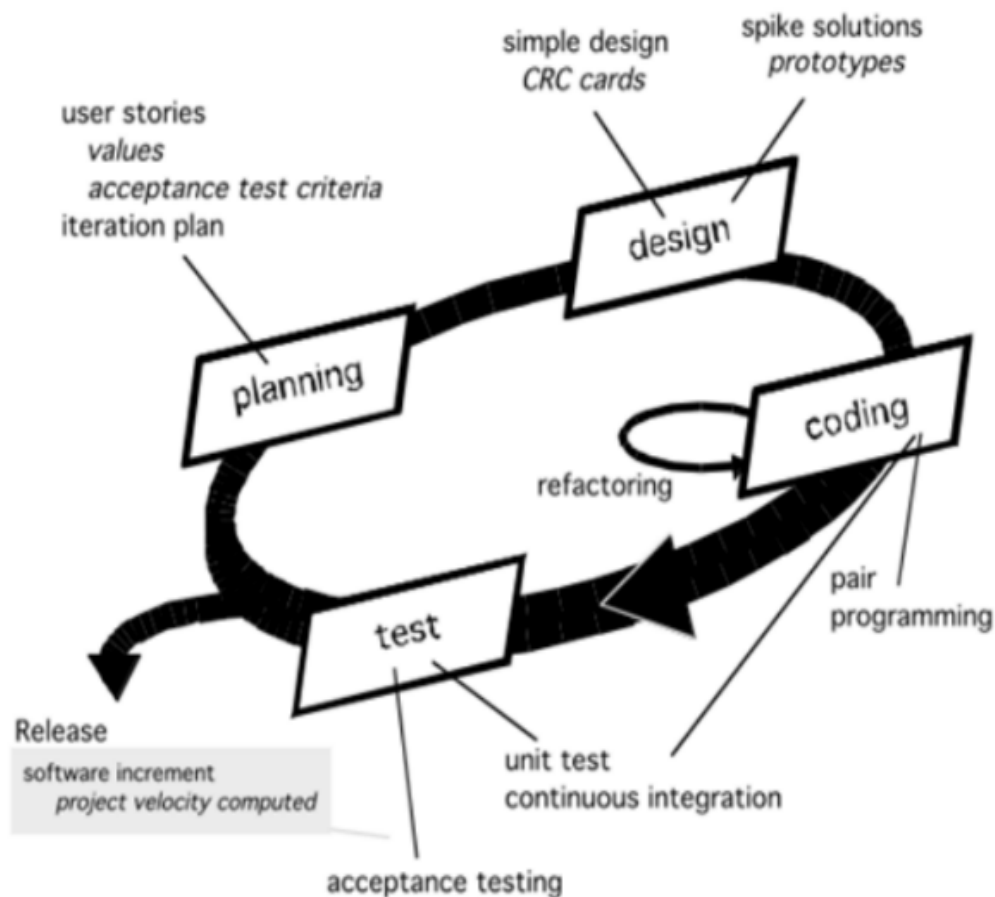
Gambar 3. 1 Extreme Programming . 48
