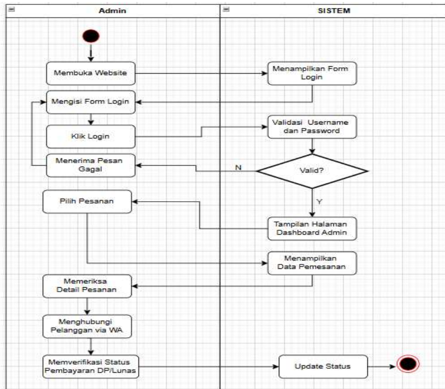
Gambar 3.2.3 Activity Diagram Admin
