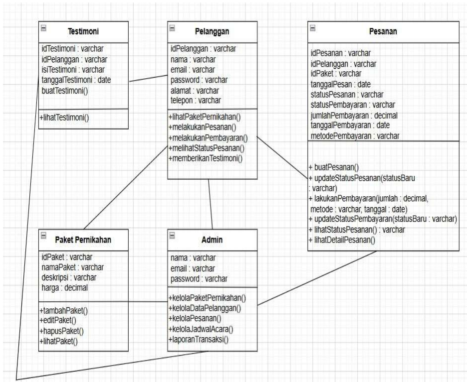
Gambar 3.3 Class Diagram
