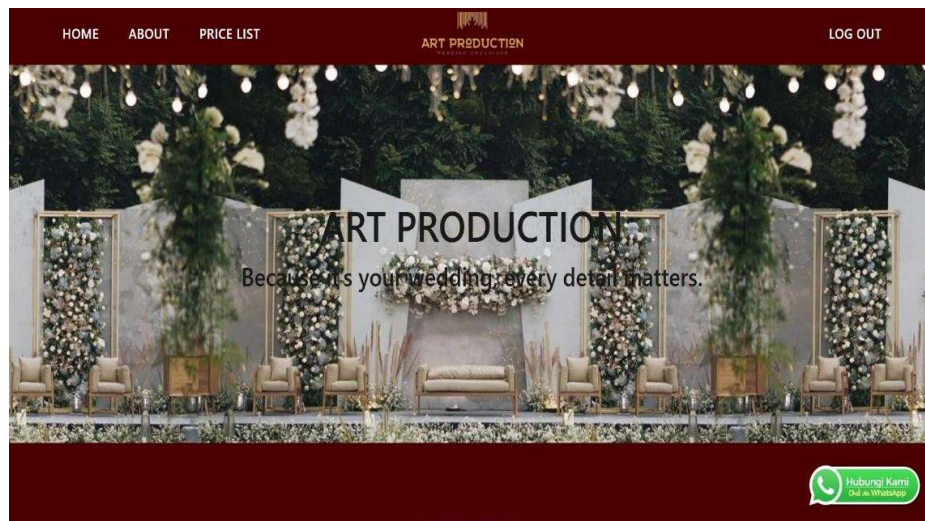
Gambar 4.1.3 Home
