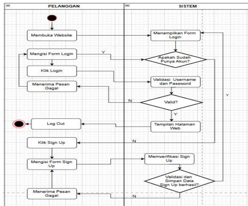
Gambar 3.2.1 Activity Diagram Login
