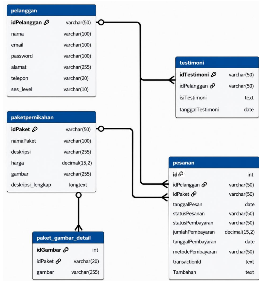
Gambar 3. 12 Entity Relationship Diagram
