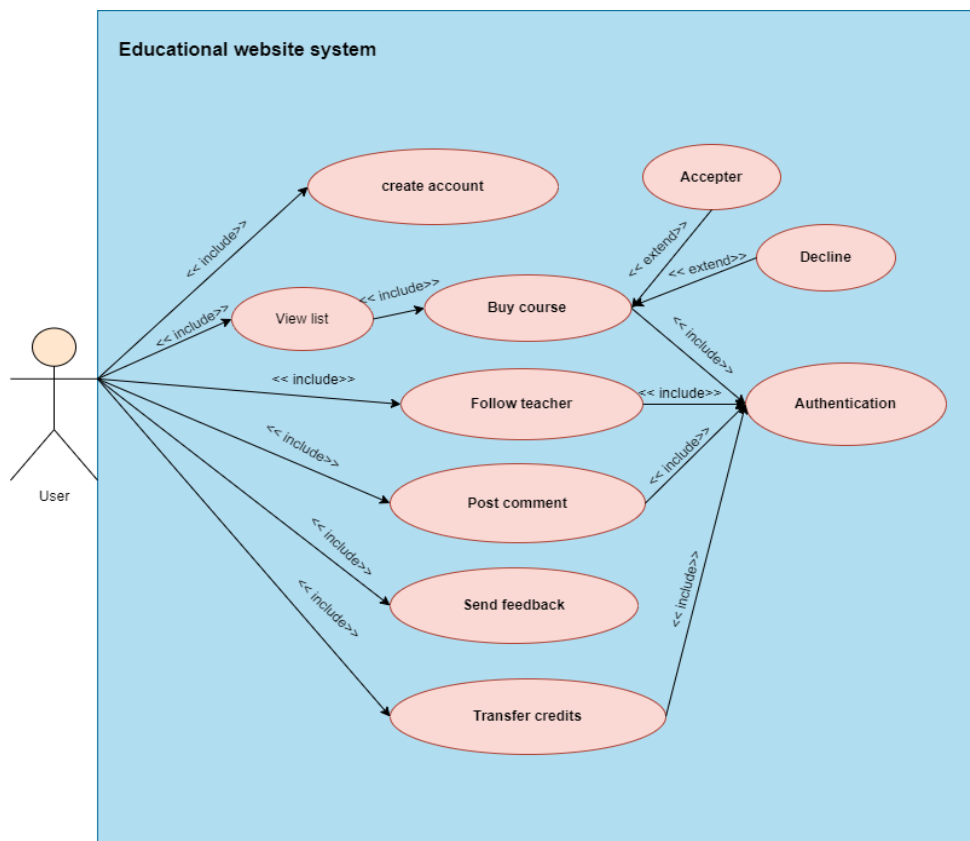
Figure 1.1 : Use case diagram for user.
