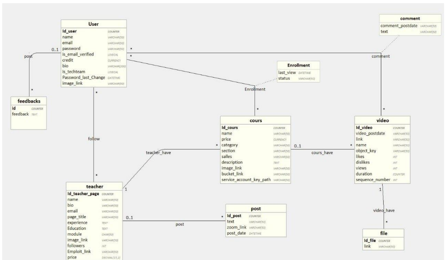
Figure 1.3 : The UML diagram of "Schooline".
