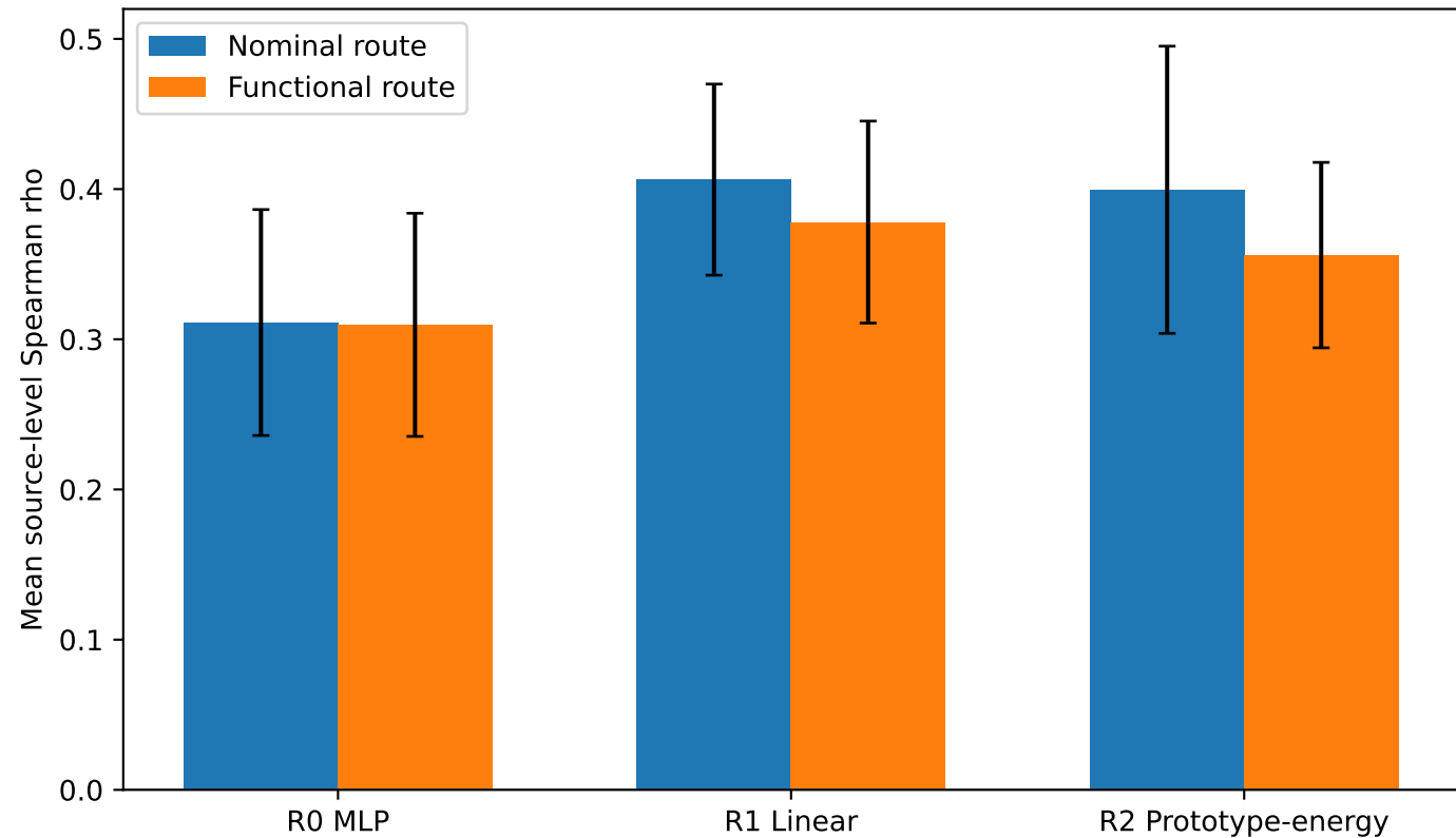
Route geometry across five model seeds
