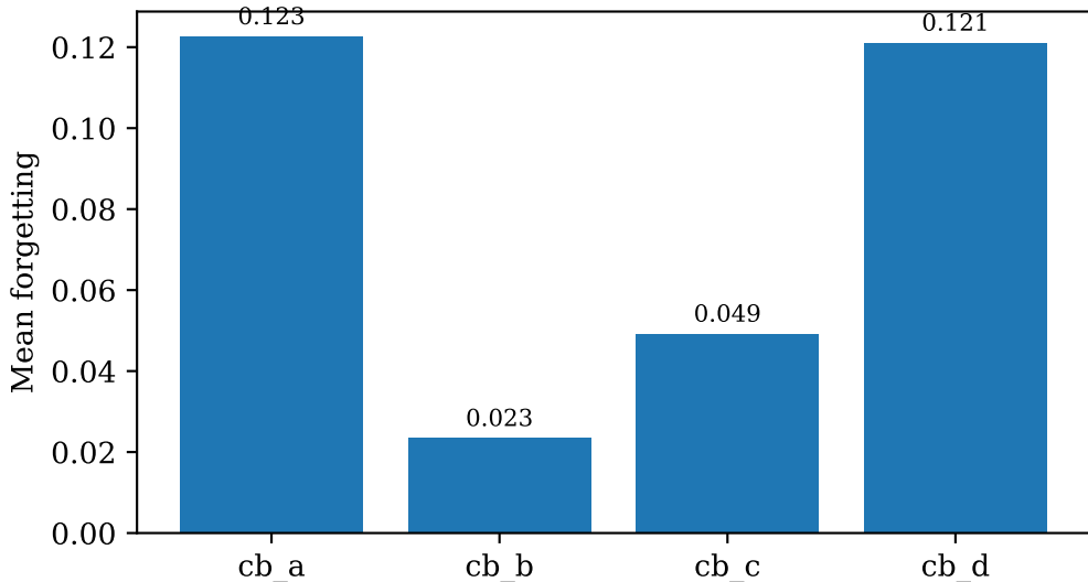
Curriculum order remains a dominant factor
