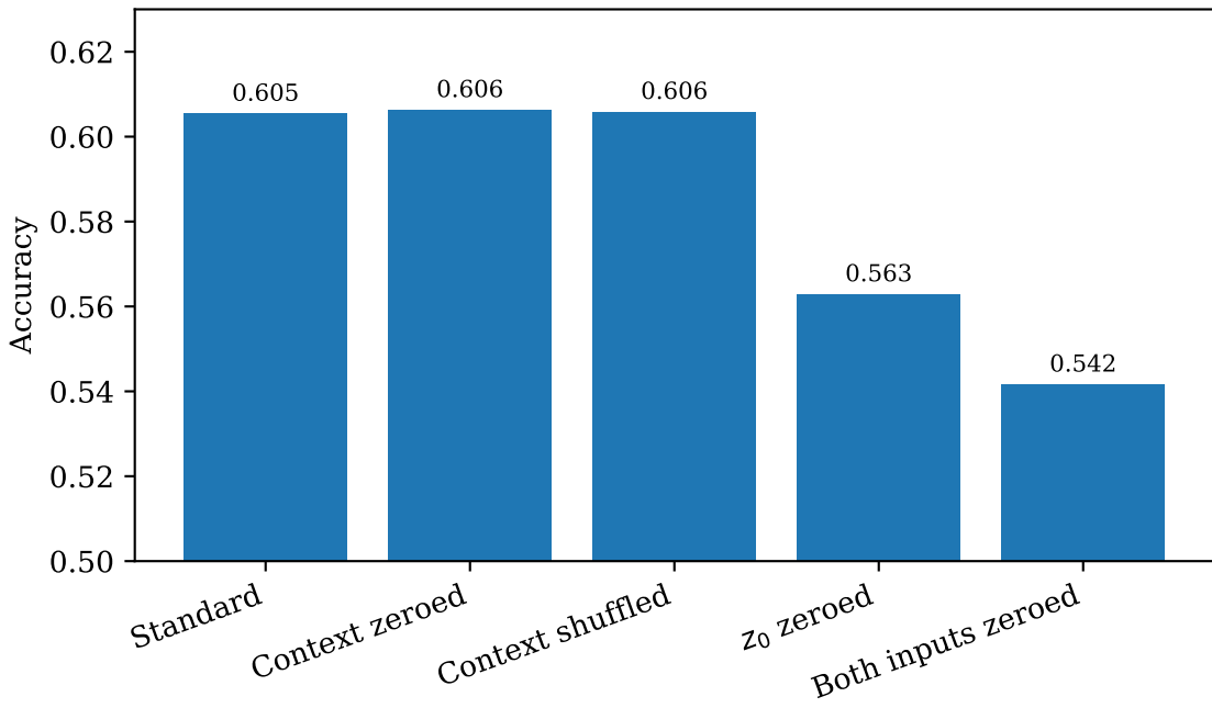
Router mediation interventions (geometry + anchor model)
