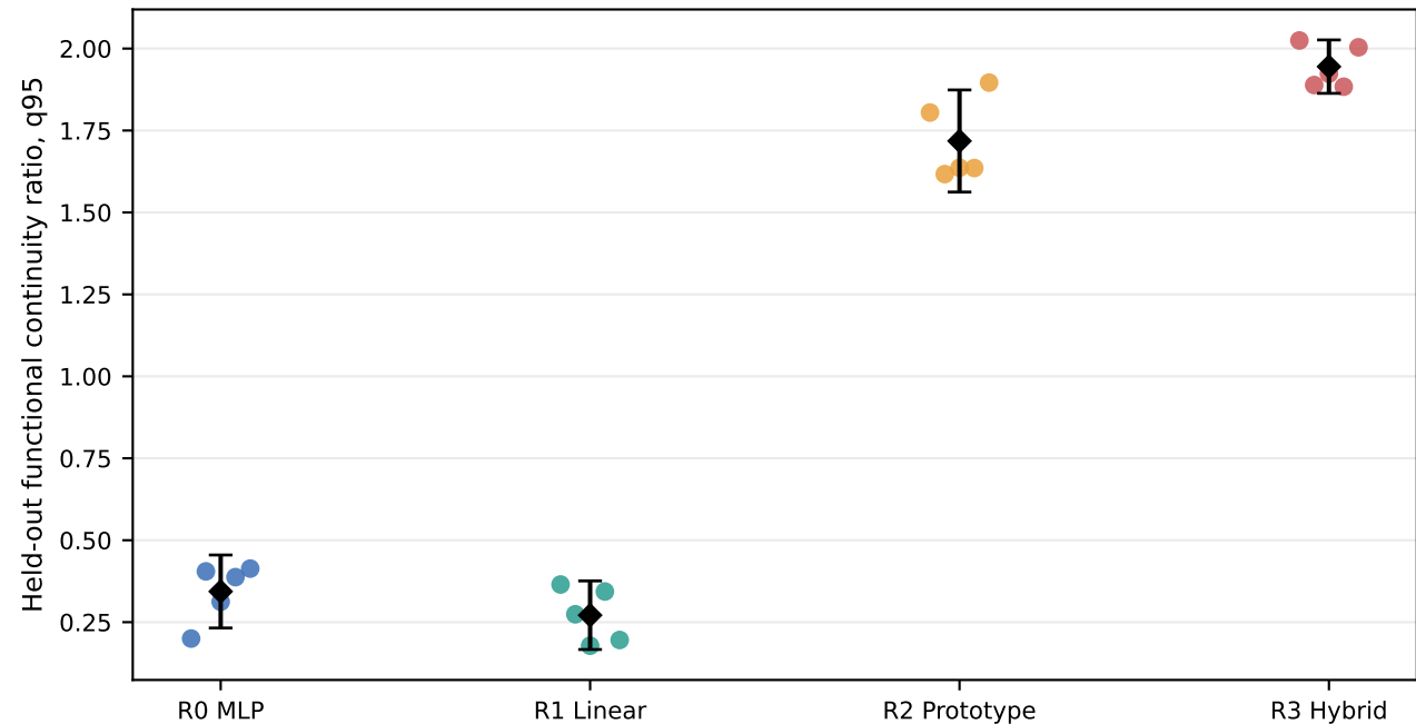
Prototype-based routers are much less locally continuous
