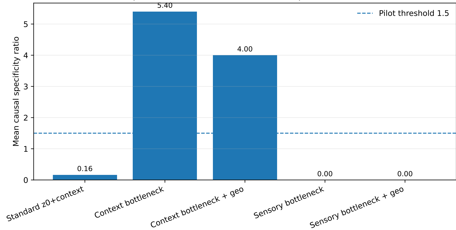
Causal probe: context bottleneck creates specific route control
