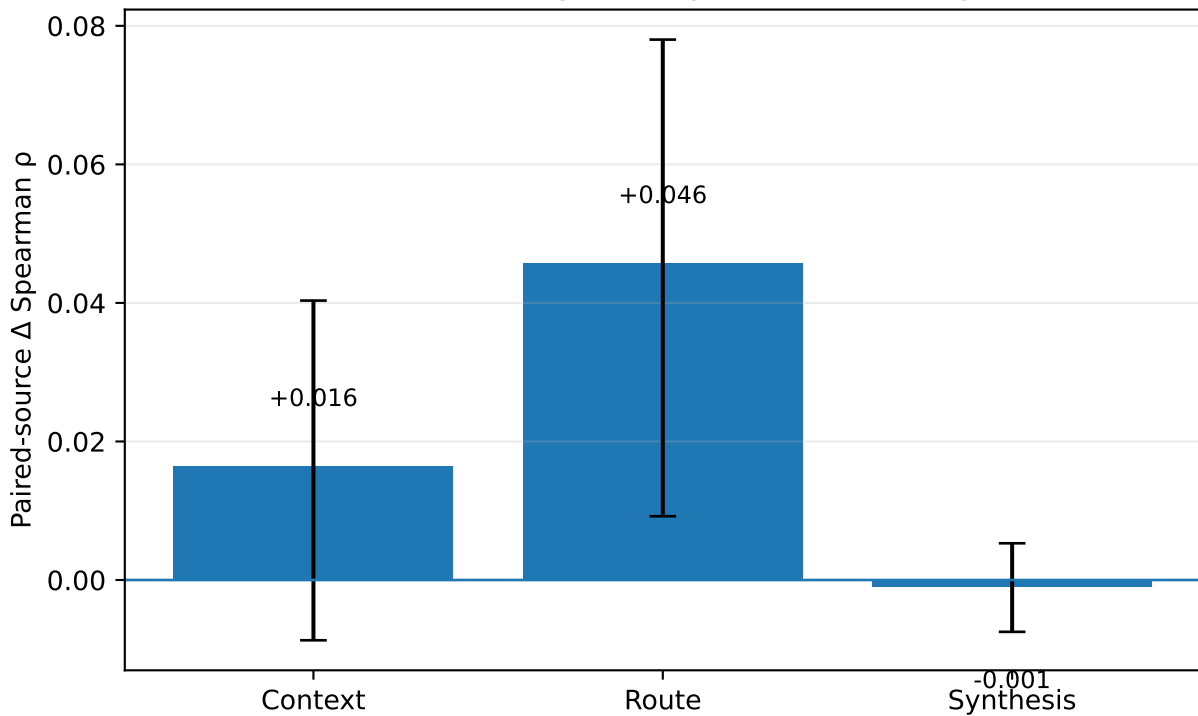
Context-bottleneck geometry effect: C2 interpolation
