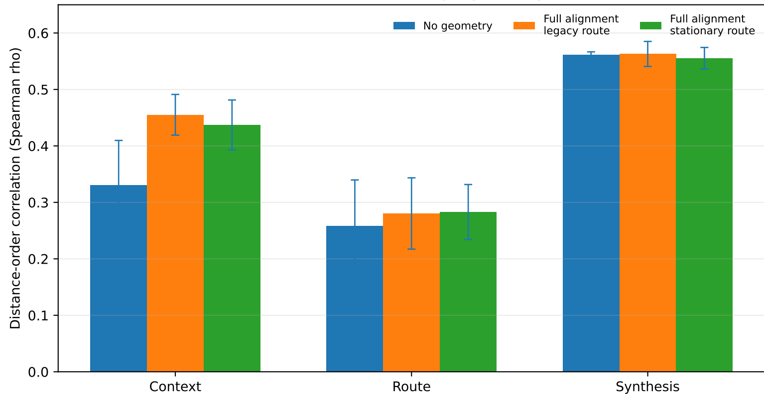
Five-seed trained-angle geometry
