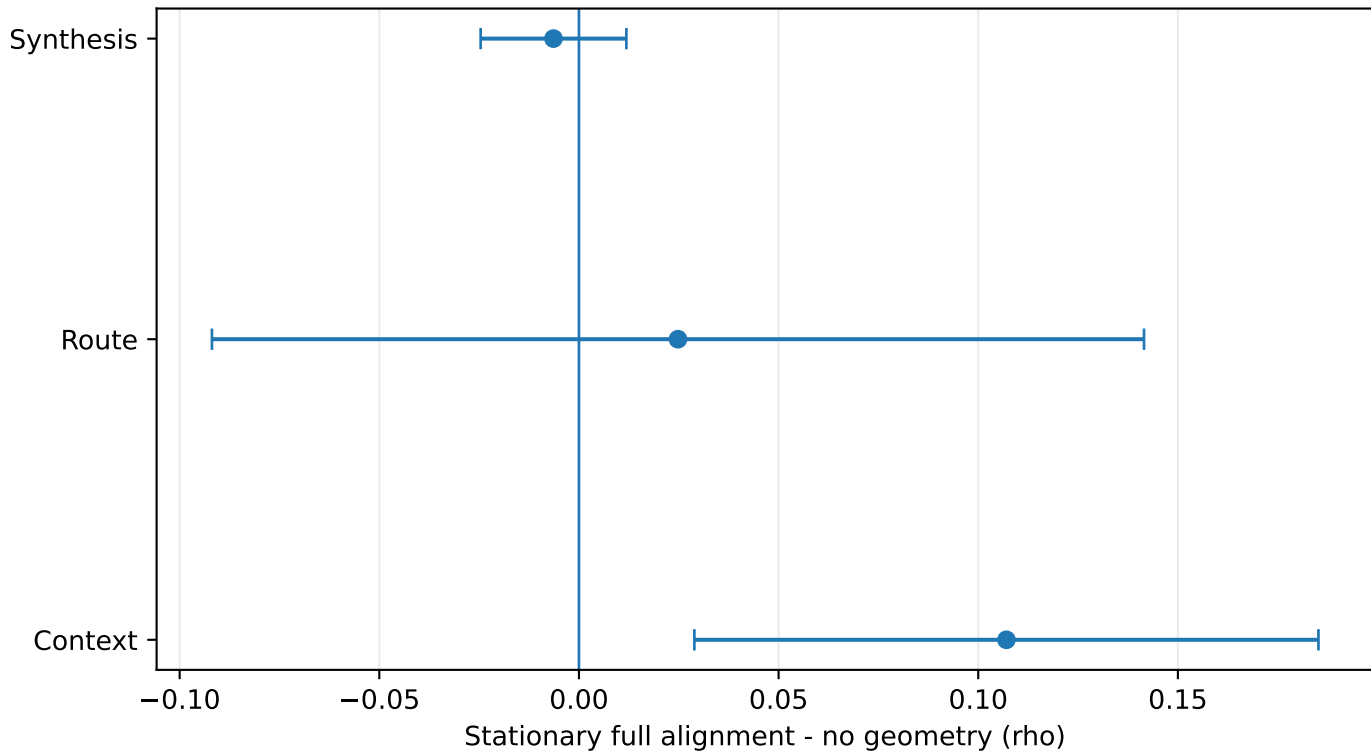
Replicated geometric effects across model seeds
