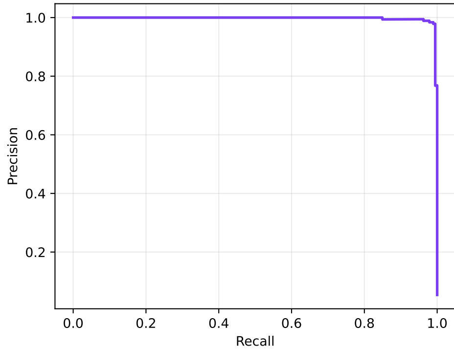
Fraud-risk precision-recall
