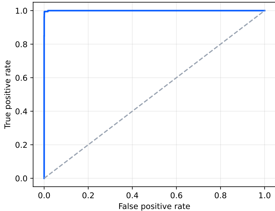
Fraud-risk ROC
