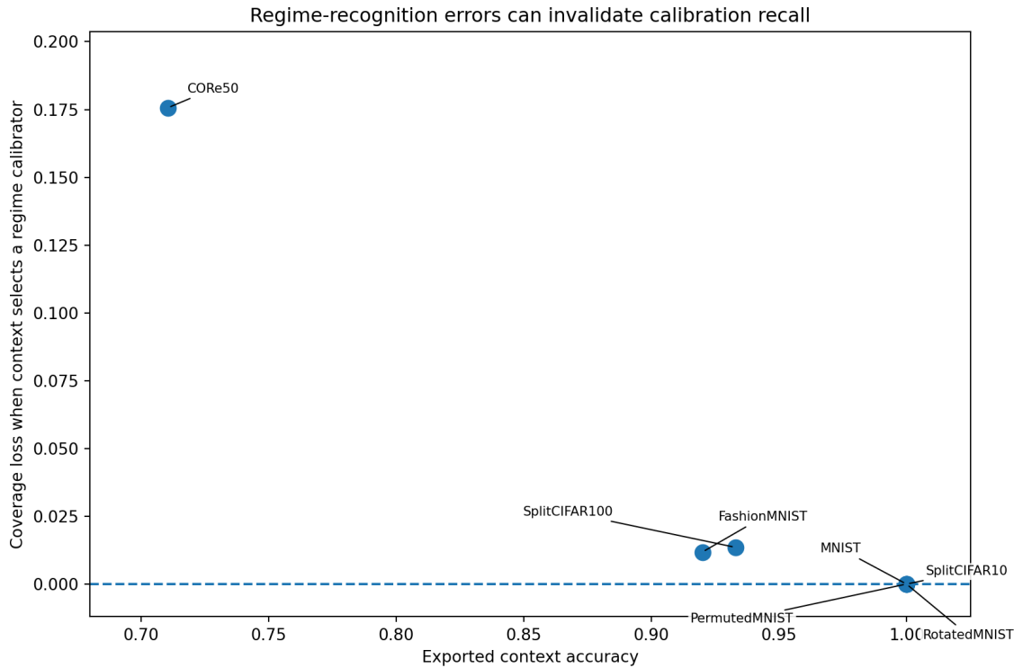
Figure 6: Context errors translate into calibration-recall loss.
