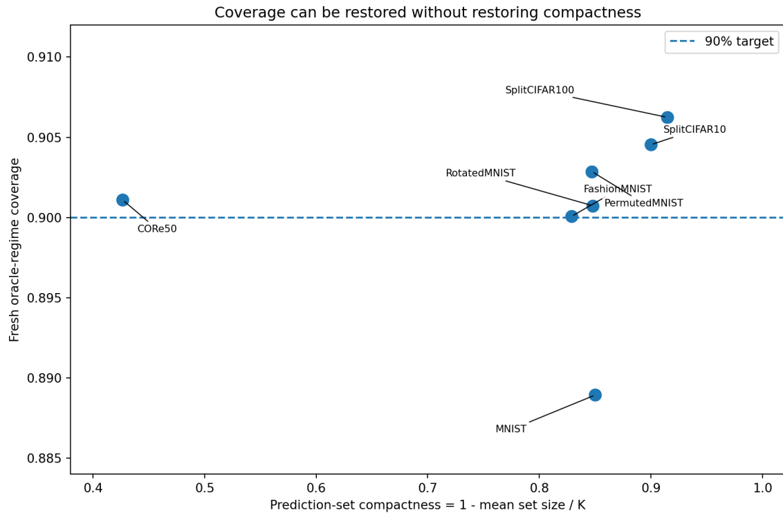
Figure 3: Coverage may be restored without restoring compactness.
