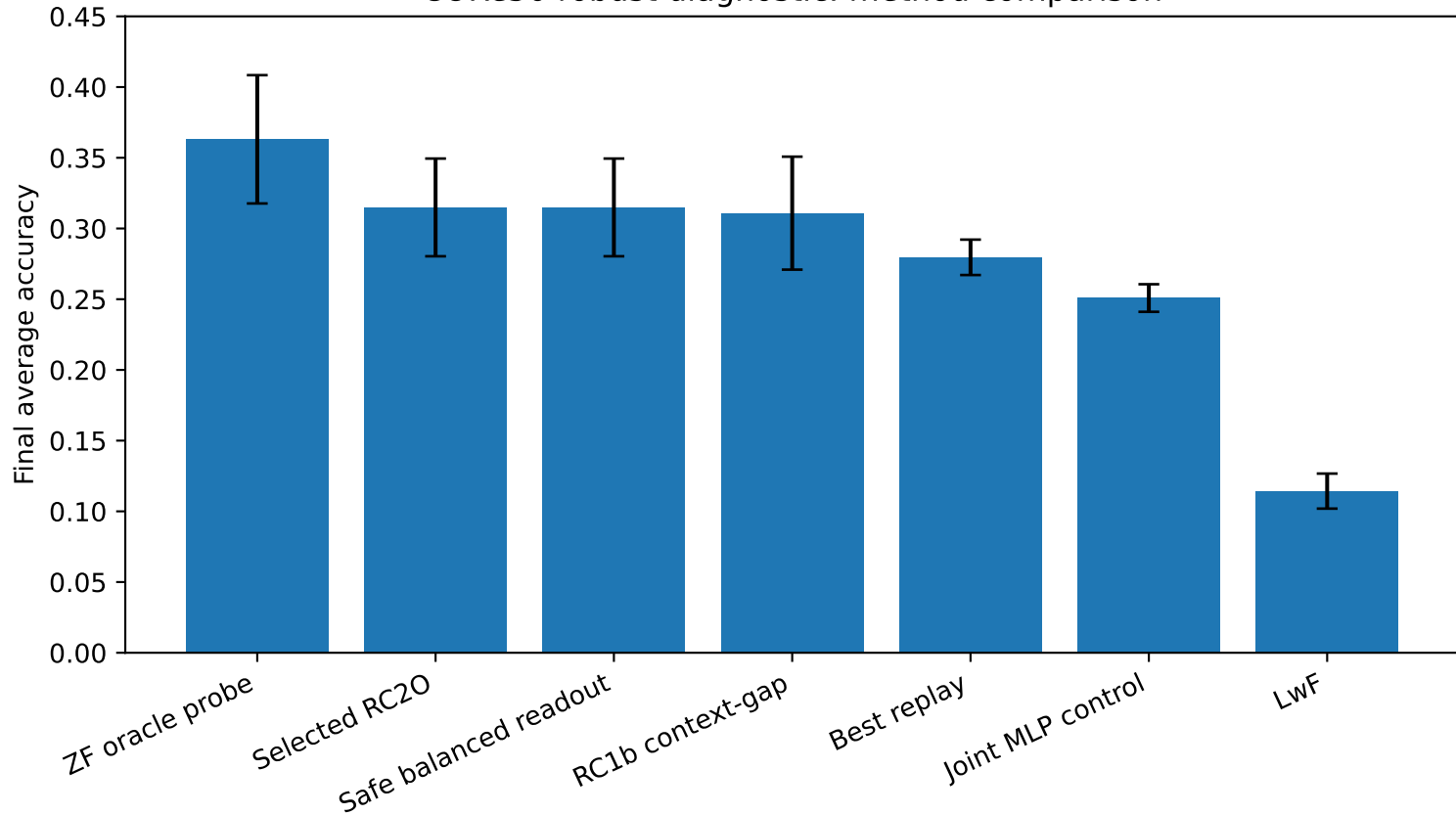
CORe50 robust diagnostic: method comparison
