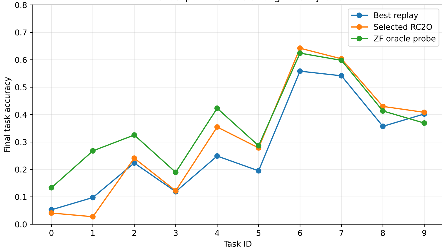
Final checkpoint reveals strong recency bias
