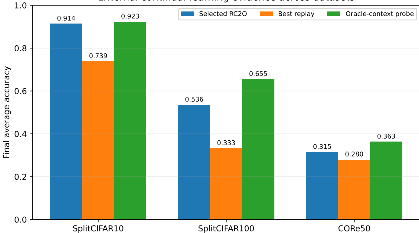
External continual-learning evidence across datasets
