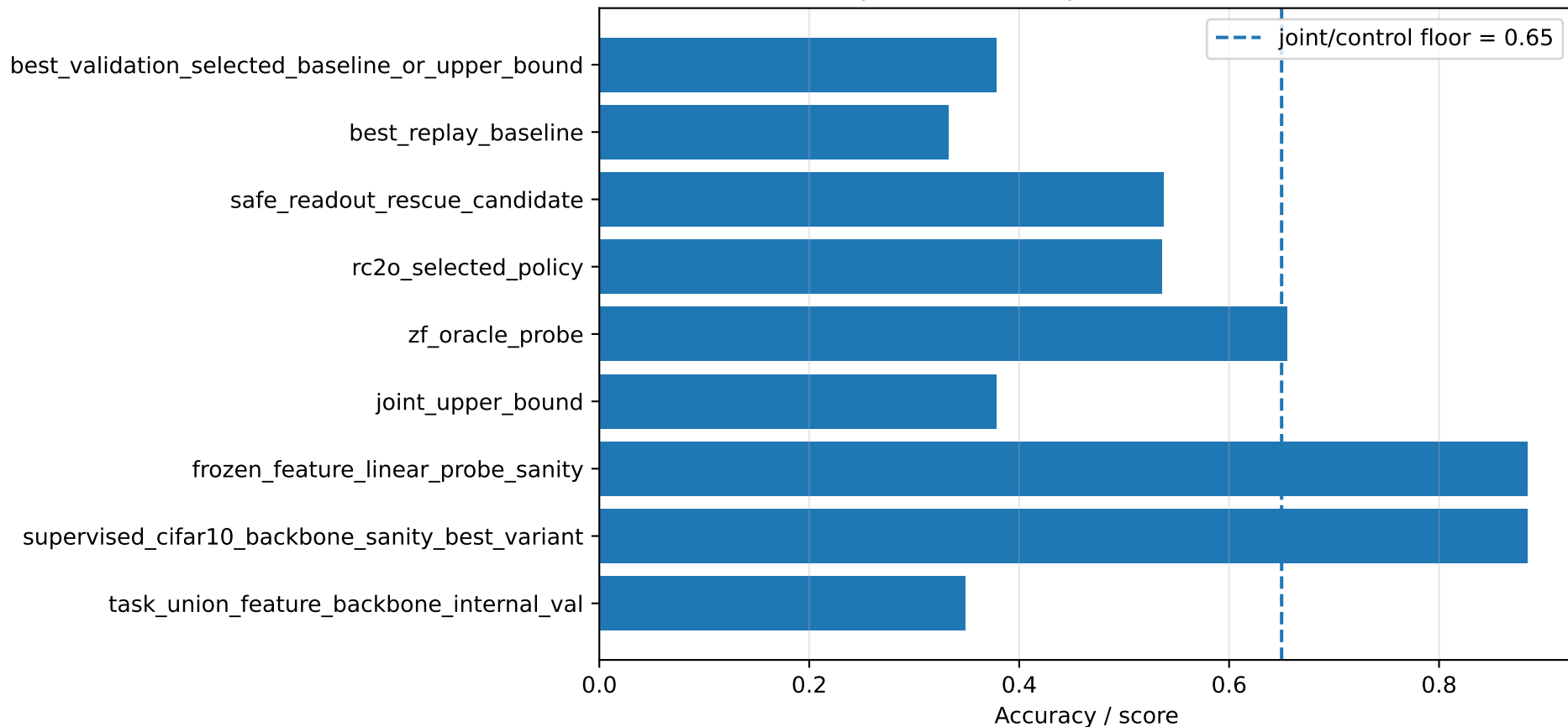
SplitCIFAR100 representation ladder
