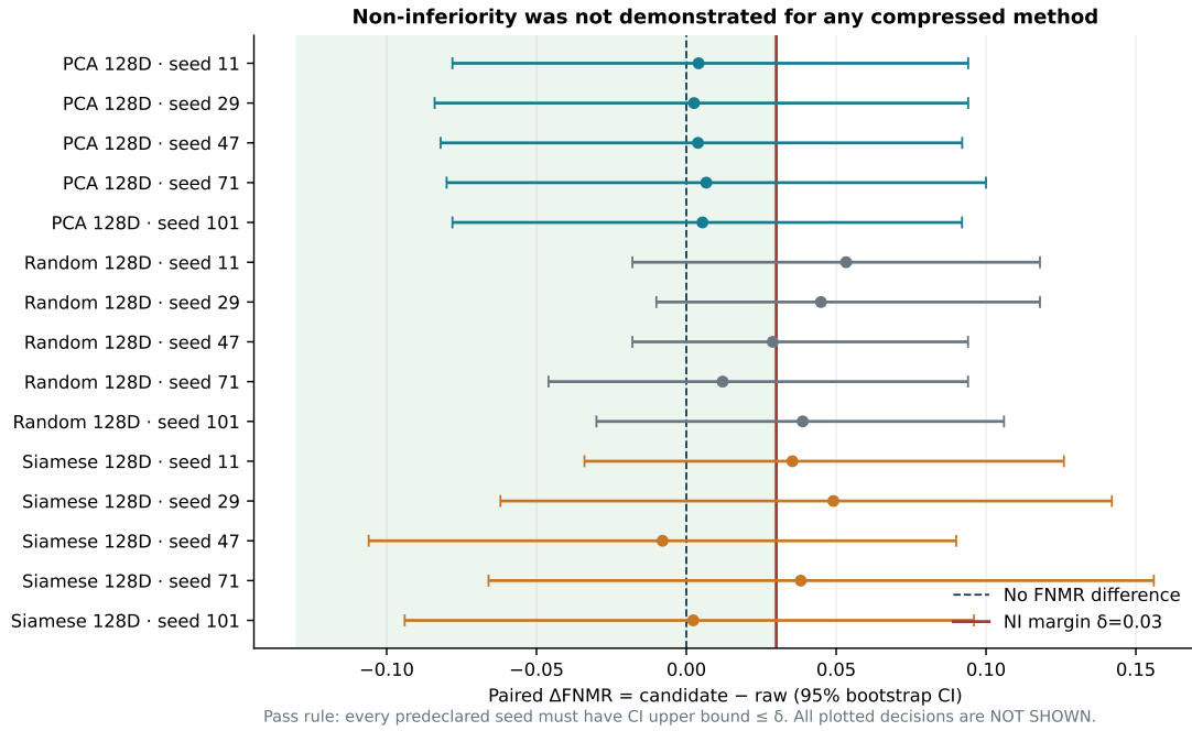
Figure 6: Seed-level paired non-inferiority analysis generated from paired_noninferiority.csv . A method passes only if the upper confidence bound is at or below \delta = 0.03 for every predeclared seed; none passes.
