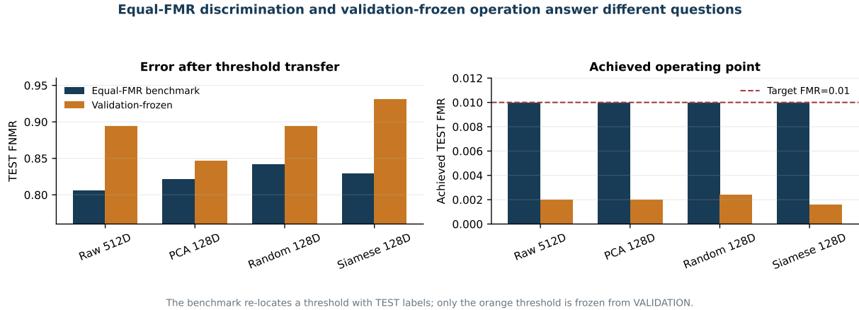
Figure 7: Threshold-transfer diagnostic generated from method_summary.csv . The equal-FMR TEST view compares discrimination but is non-deployable; the validation-frozen view measures transfer to TEST.
