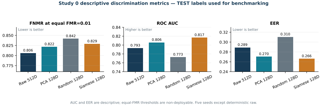
Figure 5: Descriptive Study 0 benchmark metrics generated from method_summary.csv . EER and AUC are secondary descriptions; they do not override the predeclared FNMR non-inferiority decision.
