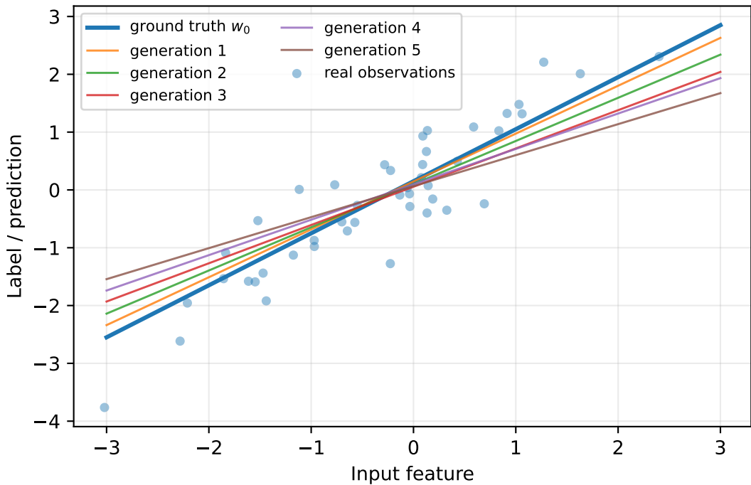
Recursive relabeling: precision can increase around a drifting target
