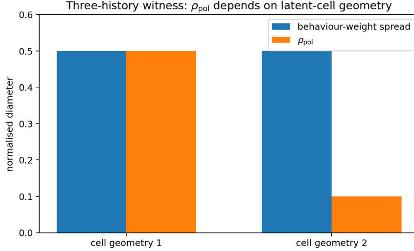
Figure 2: Same declared behaviour-weight spread, different \rho_{\text{pol}} because the latent-cell law geometry differs. This illustrates attribution; it is not a novelty claim.
