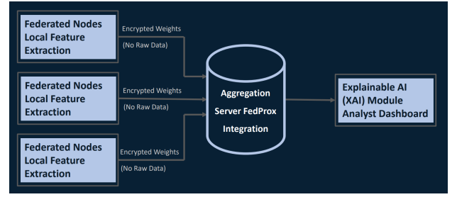
Fig. 1. Conceptual architecture of the proposed Federated Layer 2 IDS.
